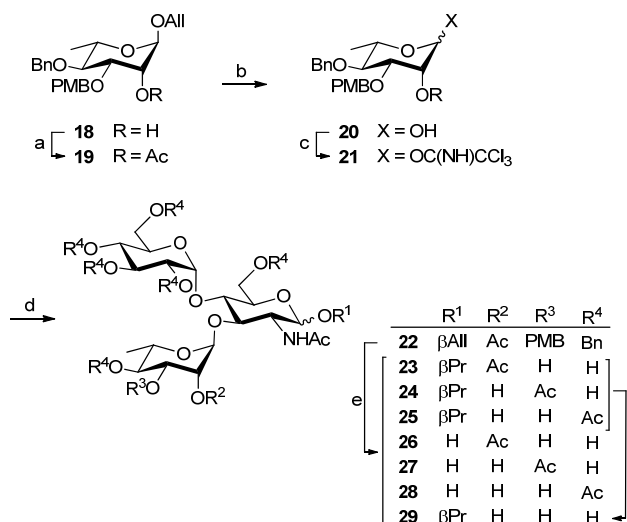
Scheme 2 Synthesis of the C(E)D-Pr trisaccharides O-acetylated at residue C or not. Reagents and conditions: a) \text{Ac}_2\text{O} , Pyr, rt, 91%; b) i. [\text{Ir}(\text{COD})\{\text{PCH}_2(\text{C}_6\text{H}_5)_2\}_2]^+\text{PF}_6^- , \text{H}_2 , THF, rt, 2 h; ii. \text{I}_2 , THF/ \text{H}_2\text{O} , rt, 1 h, 97%; c) \text{CCl}_3\text{CN} , DBU, DCE, rt, 1 h, 94%; d) 10 , Toluene, see Table 2; e) \text{H}_2 , Pd/C, 96% aq. EtOH, HCl, rt, 2 days, 47% for 23/24/25 as a 4:5:1 mix, 23% for 26/27/28 as a complex mix; f) MeONa, MeOH, rt, 69%.
