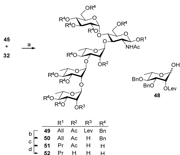
Scheme 5 Synthesis of the target pentasaccharides 51 and 52 .
