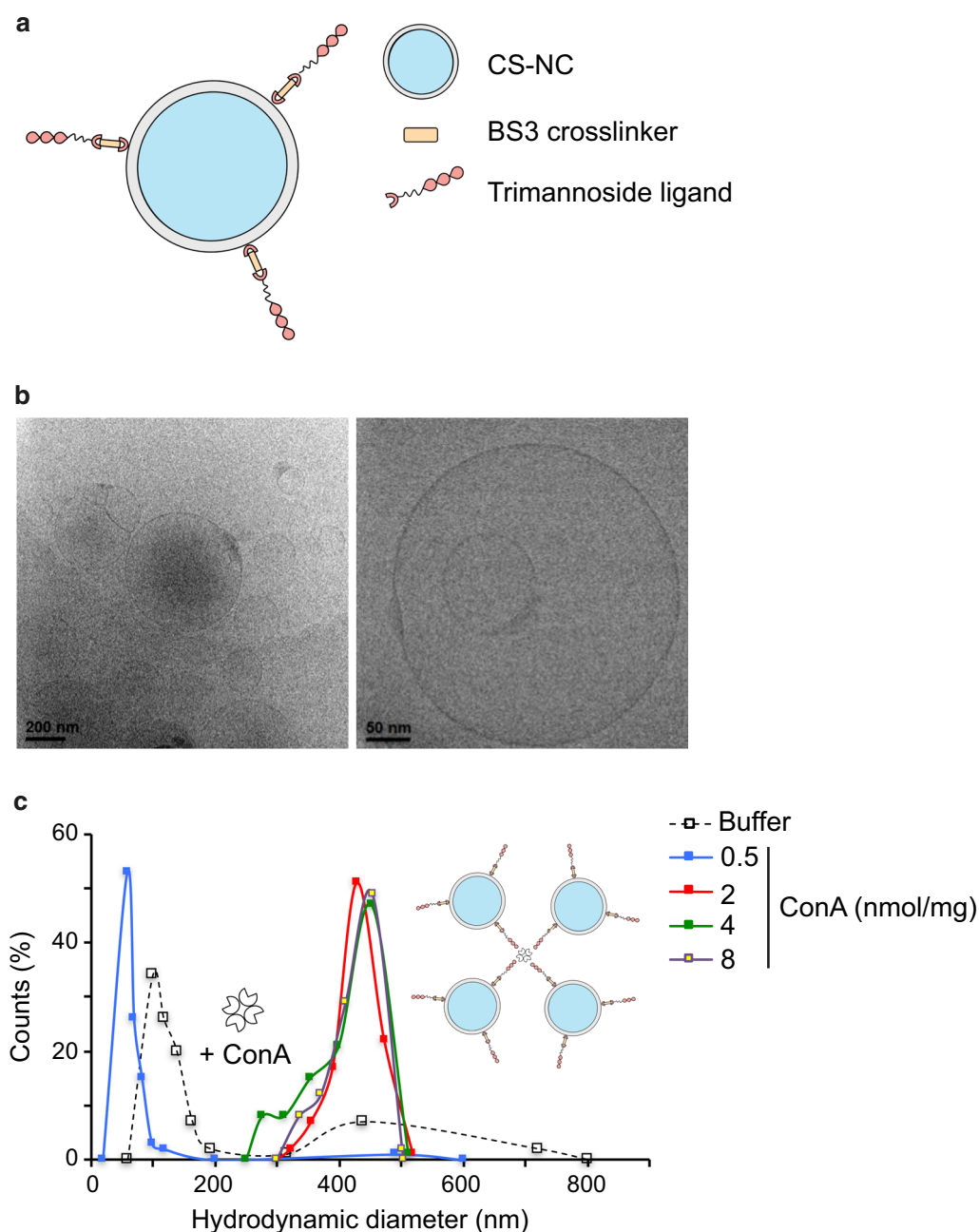
Fig. 4 Morphological characterization of tri-mannose-grafted chitosan NCs. a Schematic representation of a mannose-grafted CS-NC. b CryoTEM image of CS-NCs-tri. c Hydrodynamic diameter of CS-NCs-tri incubated at various concentrations of concanavalin A, assessed by dynamic light scattering
