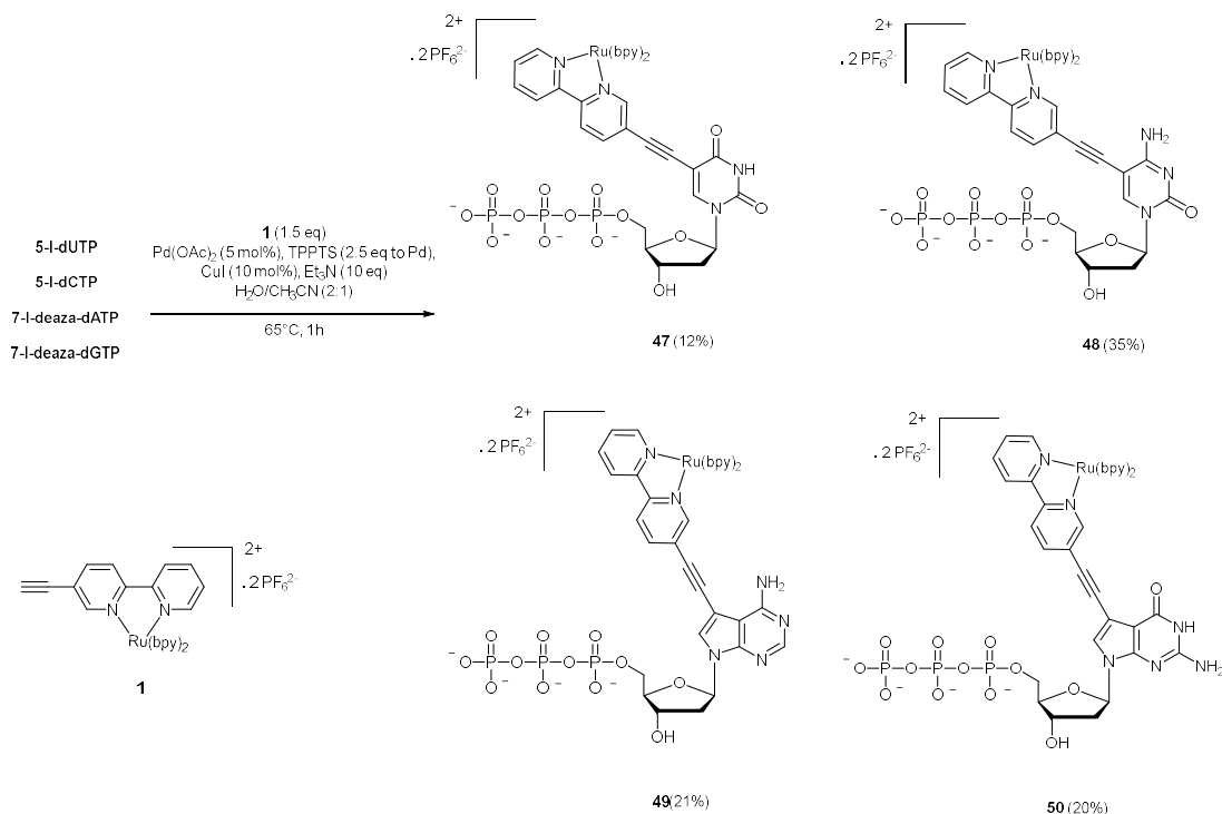
Scheme 10. Synthetic pathway for the preparation of nucleotides 47–50 [163].
