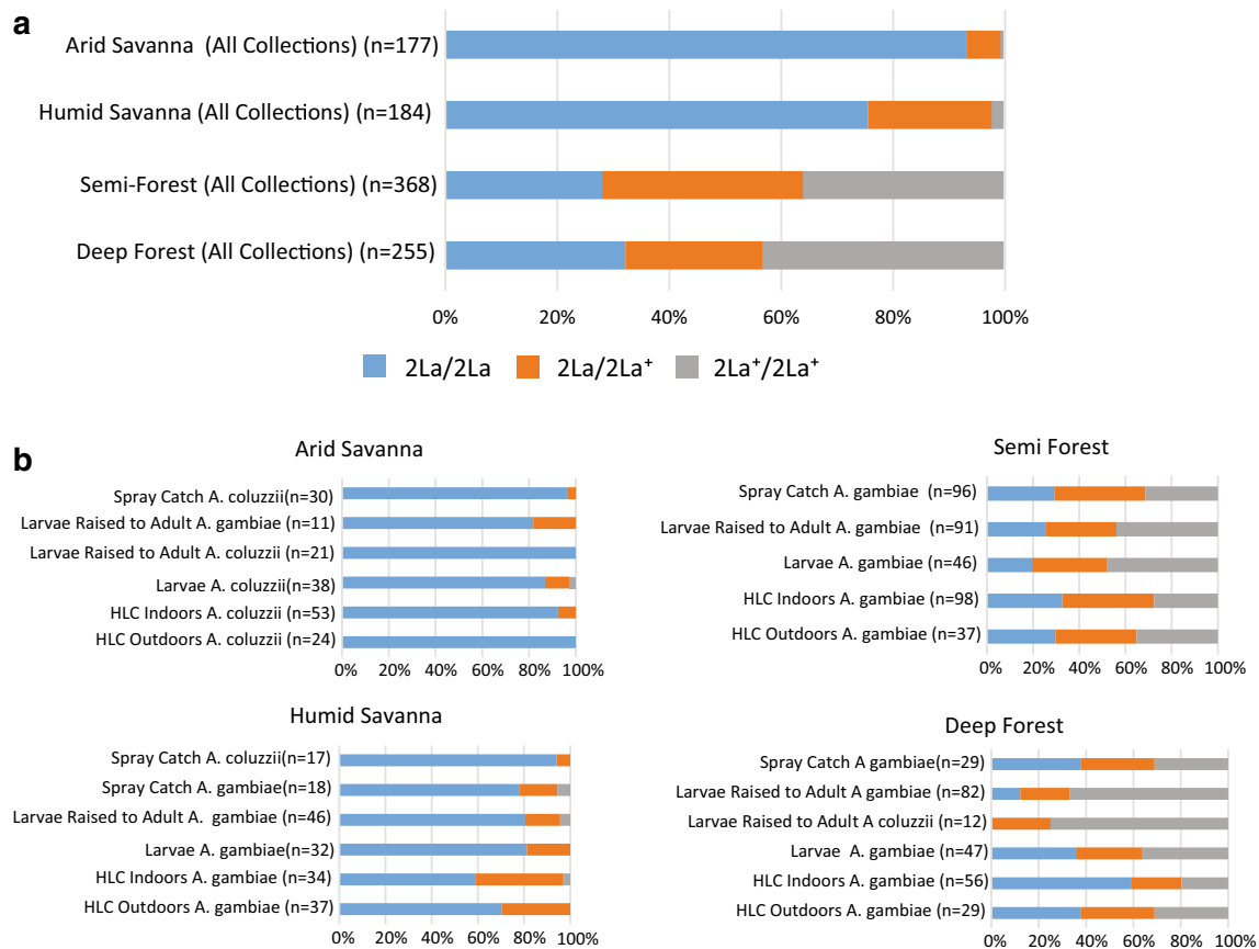
Fig. 3 Distribution of the paracentric 2La chromosome inversion. a The wild-type 2La + allele is more prevalent in forest ecologies as compared to savannah ecologies. The frequency of 2La + alleles appears to follow an ecological cline. b Rates of 2La alleles per study site by collection methodology. In the arid and humid savannah sites where the comparison can be made, A. coluzzii carried fewer 2La + chromosomes than sympatric A. gambiae collected by the same sampling methodology
