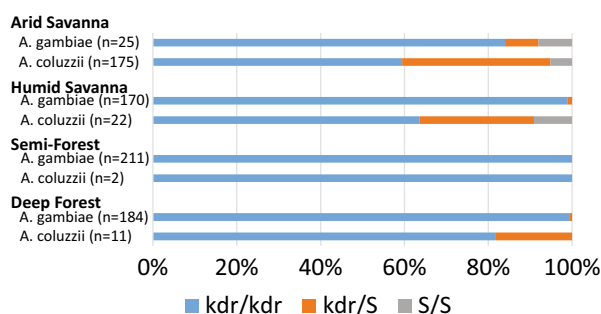
Fig. 4 The kdr-w mutation associated with insecticide resistance is nearly fixed in the vector population. The kdr-w mutation, L1014F, in the para sodium ion channel gene is prevalent across all sites. Samples from deep forest and semi-forest sites are essentially fixed for kdr-w , while the wild-type allele still segregates in the arid and humid savannah. Consistent with directional introgression of a kdr -carrying haplotype from A. gambiae into A. coluzzii , frequency of the kdr-w allele was higher across sites in A. gambiae (0.99 in A. gambiae and 0.77 in A. coluzzii )
