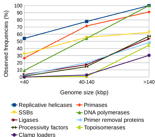
Figure 5. Relationship between the observed frequencies of viral DNA replication proteins and the genome size of dsDNA viruses.
