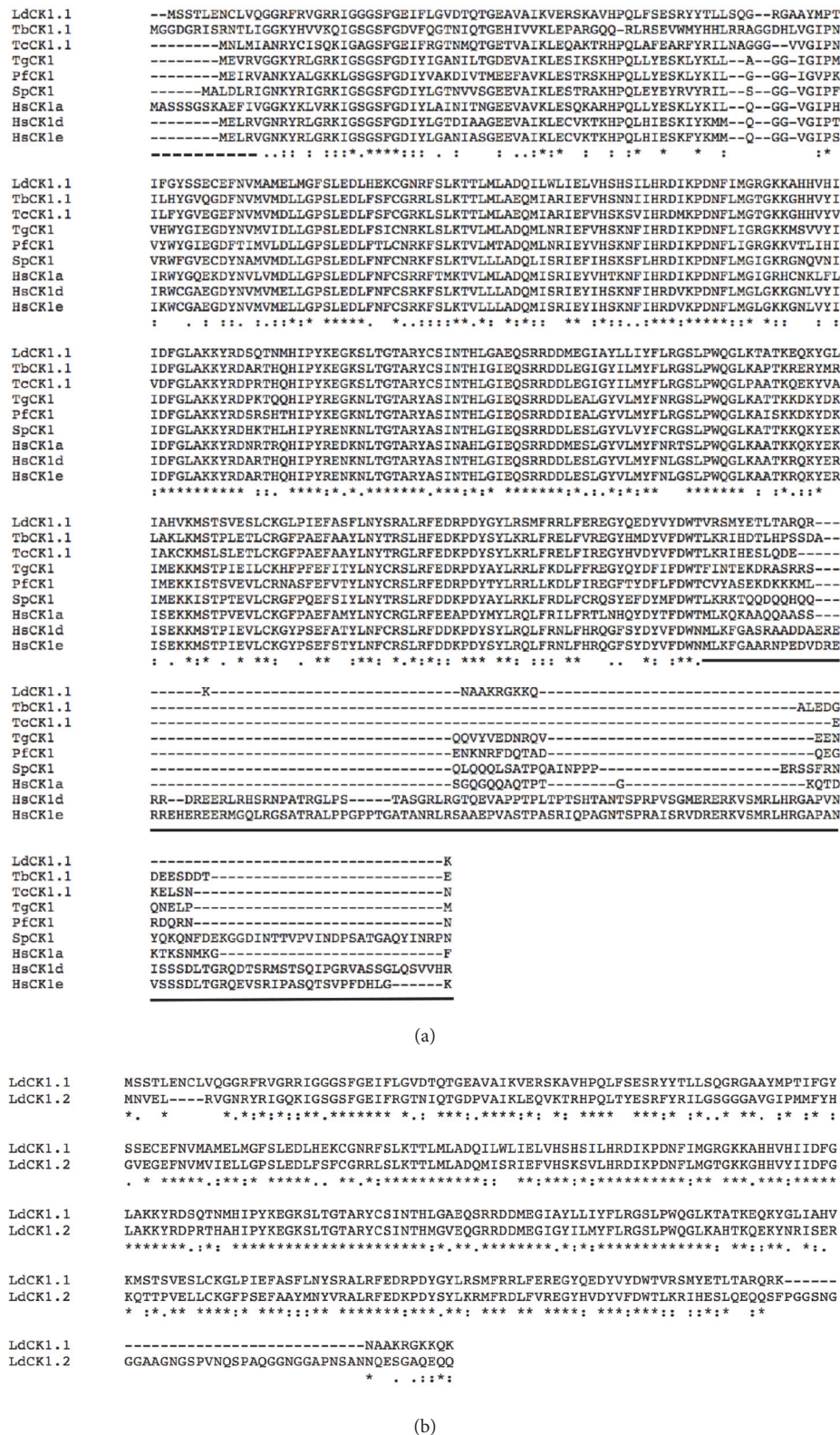
FIGURE 3: Amino acid sequence alignment of Leishmania Casein Kinase I proteins. (a) The amino acid sequences of LdCKI.1 ( Leishmania donovani LdBPK_351020.1, E9BRX8), TbCKI.1 ( Trypanosoma brucei Tb927.5.790, Q57W24), TcCKI.1 ( Trypanosoma cruzi TcCLB.508541.220, Q4DN97), TgCKI ( Toxoplasma gondii CK1, Q6QNM1), PfCK1 ( Plasmodium falciparum CK1, C6S3F7), SpCK1 ( Schizosaccharomyces pombe hhpl, P40235), hSCKI \alpha (human CSNK1A1, P48729), HsCKI \delta (human CSNK1D, P48730), and HsCKI \epsilon (human CSNK1E, P49674) have been compared and the alignments were computed using the M-Coffee mode of T-Coffee. The resulting alignments were visualized using Clustalw. * corresponds to amino acid residues that are invariant in all four CKIs. The dotted line marks the N-terminal domain, the black line marks the C-terminal domain, and the rest is the kinase domain. (b) The amino acid sequences of LdCKI.1 and LdCKI.2 (LdBPK_351030.1) have been compared and the alignments were computed using the M-Coffee mode of T-Coffee. The resulting alignments were visualized using Clustalw. * corresponds to amino acid residues that are invariant in all four CKIs.
