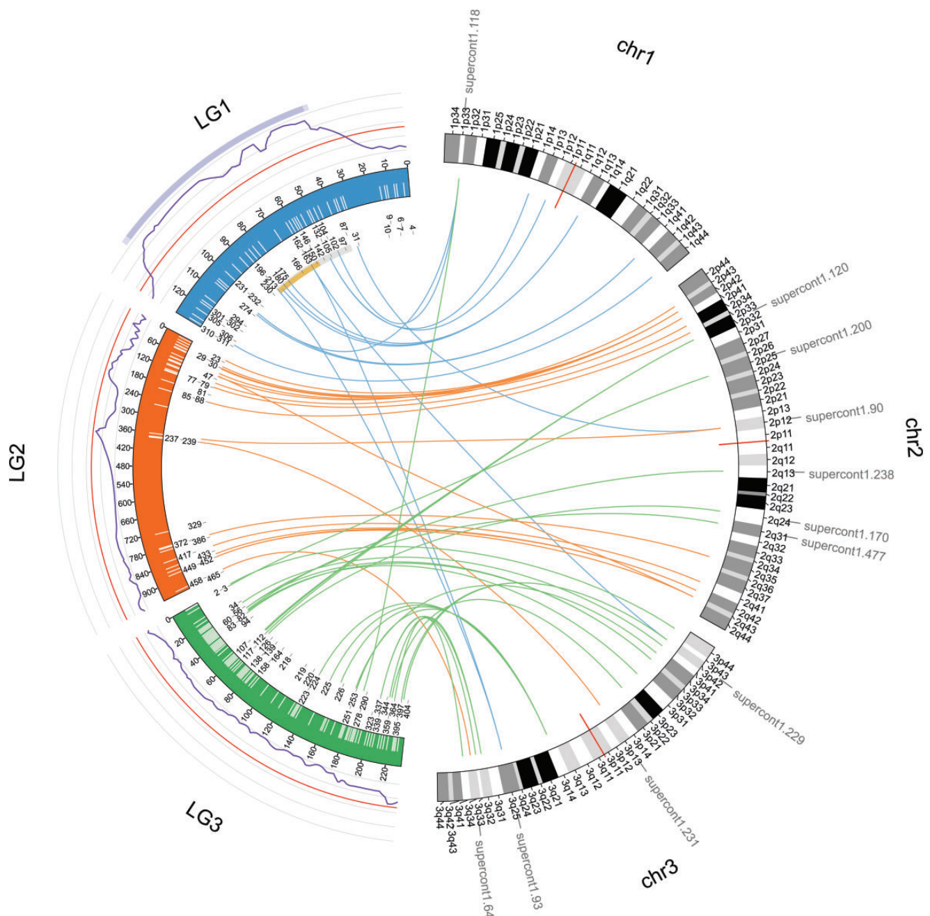
FIG. 1. —Synteny between Cross #1 linkage map and chromosome idiograms of the Aedes aegypti genome. Circos plot (Krzywinski et al. 2009) shows syntenic links between linkage (left) and chromosome (right) maps. Linkage groups (LG) are 1 (blue), 2 (orange), and 3 (green). Markers are displayed with white internal ticks with position (cM) on the scale. The genetic length of LG2 is over-inflated likely due to strongly distorted genotype segregation ratios in the centromeric part. Physical marker positions in Mbp refer to the Aaegl4 assembly coordinates and are represented below the linkage map. The LOD curve for the sex QTL is displayed in purple in the outer track of the linkage map, with the red line representing the genome-wide statistical significance threshold. LOD of 1.5 (dark purple) and 2 (light purple) support intervals are on the top. Centromeres are indicated with red ticks on the chromosome idiograms. Supercontigs with conflicting locations between the genetic and the chromosome maps are shown in grey next to the chromosome map. The 63-Mbp genomic region displaying high male–female genetic differentiation in the population data is delineated with a gold strip below LG1. The 123-Mbp region with undetectable recombination between X and Y chromosomes in both intercrosses is represented by the gold and the grey strips combined.
