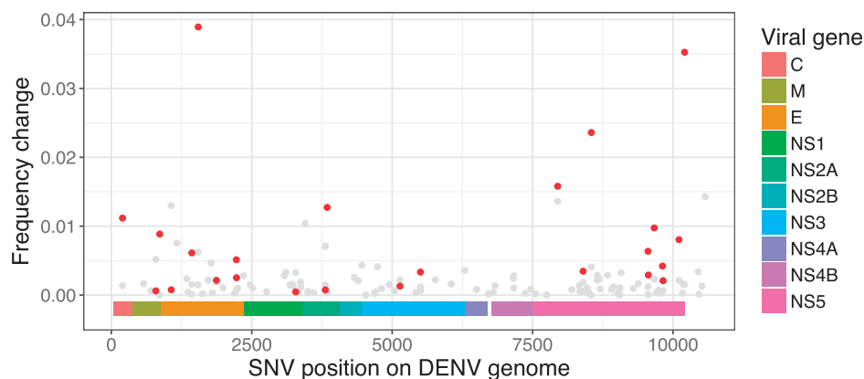
Figure 3. Change in minority variant frequency during transmission by mosquitoes. The absolute change in frequency between input (blood-meal and output (pooled saliva) samples is shown for all SNVs detected along the DENV genome. Red circles represent shared SNVs between input and saliva samples for the Gen. IV virus isolate on day 10 in Experiment A. Gray circles represent shared SNVs between two technical replicates of the input sample, as an estimate of measurement error. C, capsid protein; M, membrane glycoprotein; E, envelope glycoprotein; NS1, non-structural glycoprotein 1; NS2A, non-structural protein 2A; NS2B, non-structural protein 2B; NS3, non-structural protein 3 (protease/helicase); NS4A, non-structural protein 4A; NS4B, non-structural protein 4B; NS5, non-structural protein 5 (RNA-dependent RNA polymerase).
