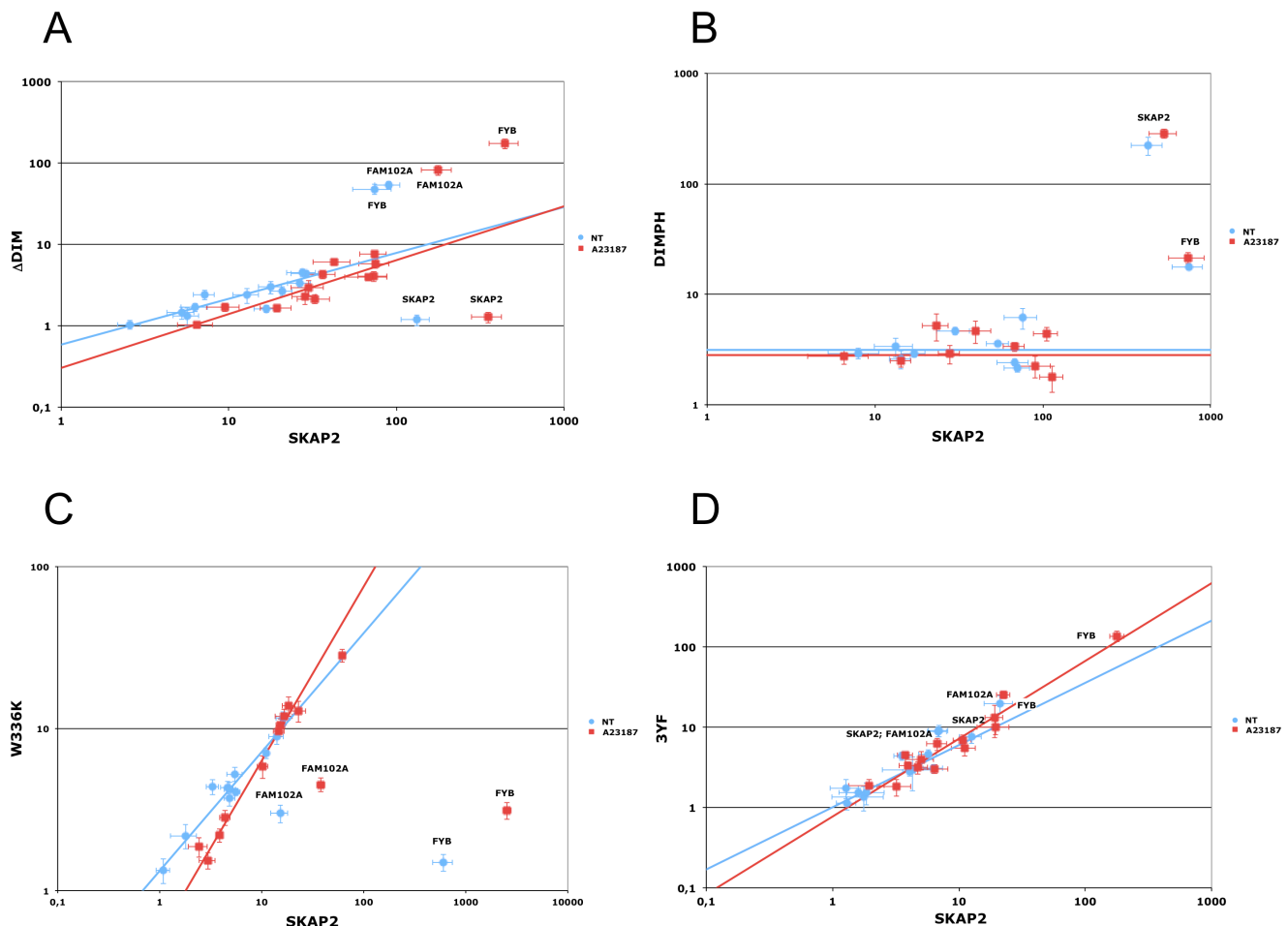
Figure 3: Edgetic effect of SKAP2 domain or binding motif inactivating mutations. Differential interaction scatterplot of SKAP2 mutant (y-axis) versus SKAP2 wild-type (x-axis) using normalized luminescence ratios are displayed in (A–D). Interactions not affected by the mutation are aligned on the diagonal. PPI disruptive mutations are located in the lower right-hand quadrant in contrast to mutations stabilizing interaction that are located on the upper left-hand one. PPI affected by the mutation are annotated. Interactions are monitored on non-stimulated (blue circle) or A23187 calcium ionophore activated (red square) cells. Error bar: Standard Error to the Mean (SEM). A robust linear regression, which takes account of outliers, was performed on data using mmregress Stata module. (A) Scatterplot comparing the interactome of SKAP2N2 and its N2-fused ΔDIM mutant. Linear regression equations are respectively \log_{10}(\Delta\text{DIM}) = 0.563 * \log_{10}(\text{SKAP2}) - 0.232 for samples without A23187 stimulation (blue line) and \log_{10}(\Delta\text{DIM}) = 0.661 * \log_{10}(\text{SKAP2}) - 0.518 for samples with A23187 stimulation (red line). (B) Characterization of the DIMPH mutant. Scatterplots compare the interactome of SKAP2N1 and its N1-fused DIMPH mutant with N1-fused SRC family members. Threshold for data without (blue line) and with (red line) activation by A23187. (C) Scatterplot comparing the interactome of SKAP2C2 and its C2-fused W336K mutant. Linear regression equations are respectively \log_{10}(\text{W336K}) = 0.733 * \log_{10}(\text{SKAP2}) + 0.124 for samples without A23187 stimulation (blue line) and \log_{10}(\text{W336K}) = 1.072 * \log_{10}(\text{SKAP2}) - 0.269 for samples with A23187 stimulation (red line). (D) Scatterplot comparing the interactome of SKAP2C2 and its C2-fused 3YF mutant. Linear regression equations are respectively \log_{10}(\text{3YF}) = 0.775 * \log_{10}(\text{SKAP2}) - 0.001 for samples without A23187 stimulation (blue line) and \log_{10}(\text{3YF}) = 0.968 * \log_{10}(\text{SKAP2}) - 0.111 for samples with A23187 stimulation (red line).
