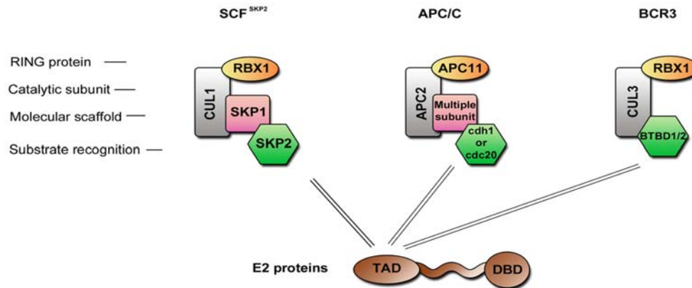
Fig. (5). Cullin-based E3 ubiquitin ligase complexes. Schematic representation of three E3 ubiquitin ligase complexes that have been shown to be regulated by the HPV E2 proteins.
