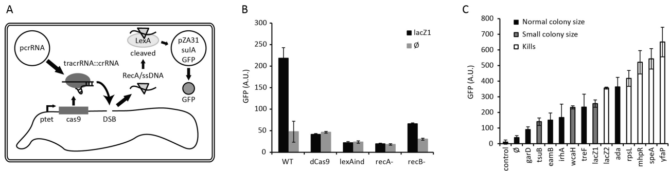
Figure 2. Cas9 cleavage in the chromosome induces the SOS response. (A) Schematic of the SOS reporter assay. Cas9 is expressed under the leaky control of a non-induced ptet promoter in the chromosome. The tracrRNA and crRNA are expressed from the pCRRNA plasmid. Cas9-mediated breaks lead to the formation of recA /ssDNA filaments which activate the self-cleavage of the LexA repressor. This releases the repression of GFPmut2 controlled by the sulA promoter. (B) The pCRRNA plasmid programmed to target the lacZ1 position (black bars) or a control empty pCRRNA (gray bars) were introduced in different cell backgrounds. GFP fluorescence was measured during exponential growth (mean \pm s.d., n \geq 3 ). (C) SOS response resulting from CRISPR targeting with different spacers. The bar marked as 'control' indicates the auto-fluorescence level of Escherichia coli without the pZA31- sulA -GFP plasmid. Spacers that cannot be transformed under constitutive Cas9 expression from the pCas9 (see Figure 1B) are shown in white. Spacers that can be transformed but lead to the formation of small colonies (see Figure 1B) are shown in gray. Finally, spacers that can be transformed in the presence of pCas9 and form colonies of regular size (see Figure 1B) are shown in black (mean \pm s.d., n \geq 3 ).
