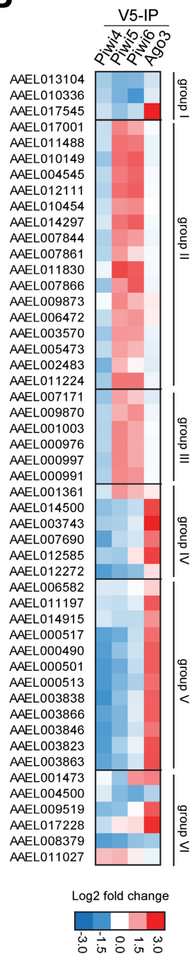
Figure 1. Genic piRNAs depend on different combinations of Aedes aegypti PIWI proteins. (A) Relative changes in piRNA abundance of the top-50 piRNA producing protein-coding genes upon PIWI knockdown. Left panel: heatmap showing the relative piRNA abundance in the indicated knockdown libraries compared to the control knockdown (dsLuc). These data were used to generate the hierarchical clustering and assign individual genes to specific groups (I–VI). The virus symbol indicate annotated genes of viral origin. Middle panel: antisense bias, defined as the percentage of antisense 25–30 nt reads that map to genic sequences. Right panel: nucleotide bias at each position of the 25–30 nt small RNA reads mapping to the sense (upper panels) and antisense coding gene sequences (lower panels). All reads of three independent experiments were combined to generate sequence logos using the Weblogo3 program. n , number of reads; u , number of unique sequences. (B) Heatmap showing the relative piRNA abundance in the indicated Piwi IP libraries over the control IP (GFP).
