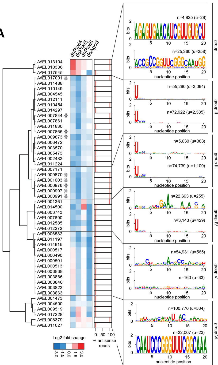
Figure 1. Genic piRNAs depend on different combinations of Aedes aegypti PIWI proteins. (A) Relative changes in piRNA abundance of the top-50 piRNA producing protein-coding genes upon PIWI knockdown. Left panel: heatmap showing the relative piRNA abundance in the indicated knockdown libraries compared to the control knockdown (dsLuc). These data were used to generate the hierarchical clustering and assign individual genes to specific groups (I–VI). The virus symbol indicate annotated genes of viral origin. Middle panel: antisense bias, defined as the percentage of antisense 25–30 nt reads that map to genic sequences. Right panel: nucleotide bias at each position of the 25–30 nt small RNA reads mapping to the sense (upper panels) and antisense coding gene sequences (lower panels). All reads of three independent experiments were combined to generate sequence logos using the Weblogo3 program. n , number of reads; u , number of unique sequences. (B) Heatmap showing the relative piRNA abundance in the indicated Piwi IP libraries over the control IP (GFP).
