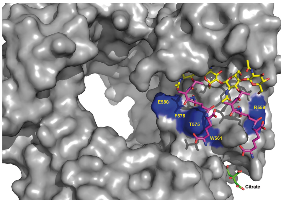
Figure 7. Model of the interaction between LtgA and chitotetraose modified with PG tripeptide stems, which terminates in a meso -DAP residue, MurNAc(L-Ala-D-Glu- meso -DAP). The model highlights the two stem peptide-binding grooves predicted to be involved in PG binding for E. coli Slt70, aligned on the conserved residues (Glu 580 , Phe 578 , Thr 575 , Trp 561 , and Arg 559 ) (Fig. 4b). A citrate molecule (colored in pink) occupies binding site –2.
