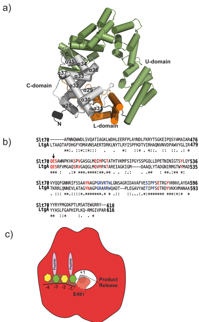
Figure 4. Native structure of LtgA. a , ribbon model of the highly helical LtgA structure, consisting of 37 \alpha -helices. LtgA has C (gray), L (orange), and U (green) domains. The C domain houses the catalytic domain. b , sequence alignment of the C domains of LtgA and Slt70. Residues predicted to be involved in glycan chain binding and/or catalysis are highlighted in red, and residues predicted to be involved in PG stem peptide interactions are highlighted in blue. An arrow points to the conserved catalytic glutamate of LtgA and Slt70. LtgA shares 25% sequence similarity with the C domain of Slt70. The asterisk indicates absolute conservation, and the dots (.) indicate high conservation. c , three bona fide binding subsites lie in the protein interior and are labeled -1 to -3. Subsite -4 is at the entrance of the active site, whereas subsite +1 lies at the exit of the active site. Subsites +1 and -1 are buried and protected from the solvent and are closest to the catalytic residue Glu 481 . Previous studies predict binding sites -1 and -3 to be occupied by the 1,6-anhydro-MurNAc products.
