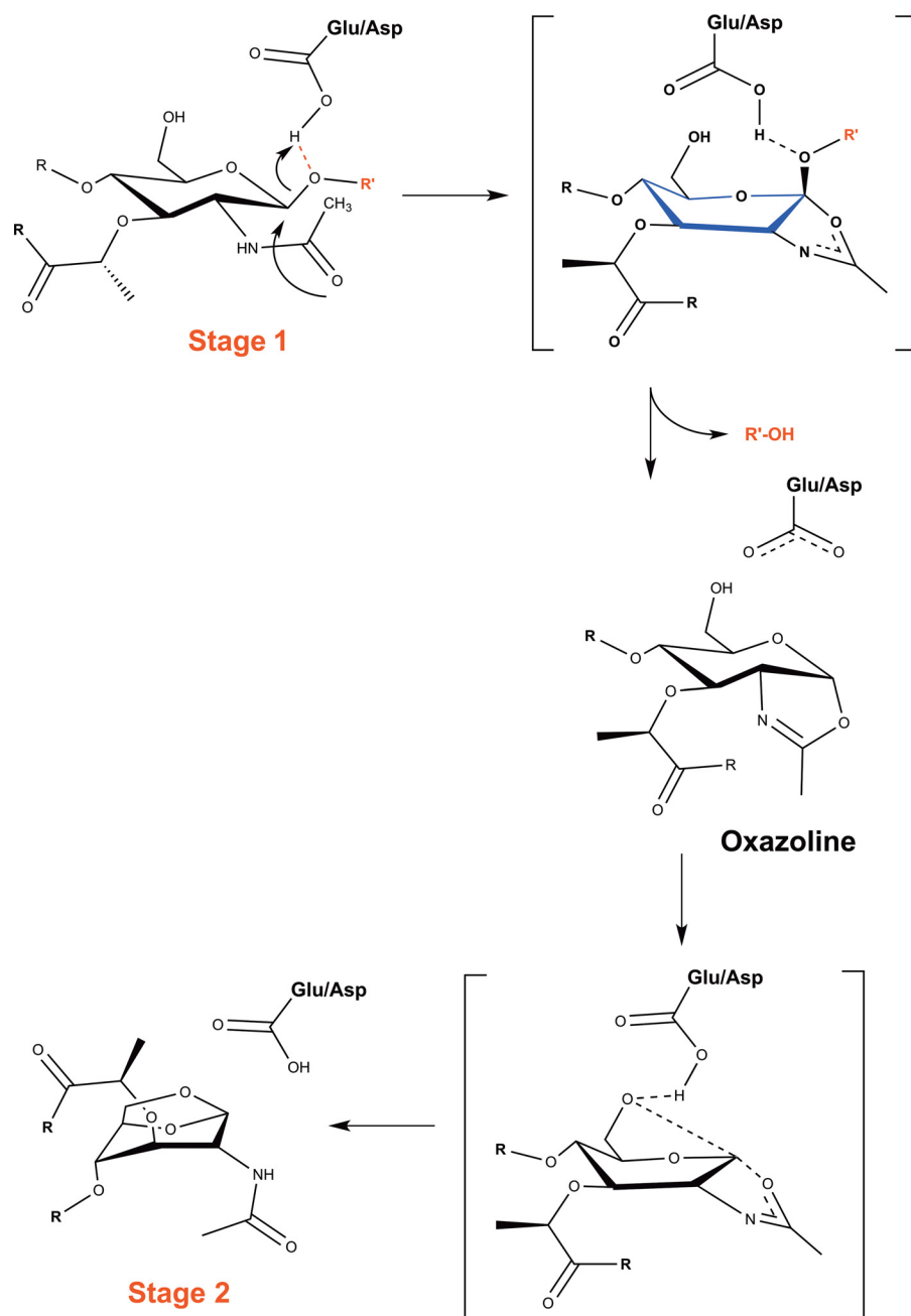
Figure 1. Proposed catalytic mechanism of LTs. LTs use a single catalytic glutamate or aspartate in a simple acid followed by base catalysis. In the absence of a second catalytic residue in the active site, these enzymes proceed via the anchimeric assistance of the MurNAc 2-acetamido group and the formation of the oxazolinium ion intermediate (32).
