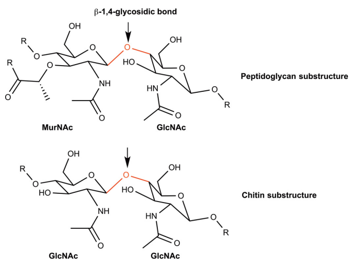
Figure 2. Comparison of the PG and chitin substructures. The \beta -1,4-glycosidic bond, which is the chemical site of LT activity, occurs in both the PG and chitin substructures.
