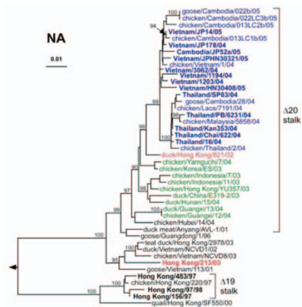
Figure 2. Phylogenetic relationships among N1 neuraminidase (NA) genes of H5N1 influenza viruses. The clade of the hemagglutinin of each of these viruses is indicated by font coloring as in Figure 1A. Brackets denote genes encoding NA protein with deletions in the stalk region; residues 49–68 for clades 1–2 and 57–75 in clade 3.
