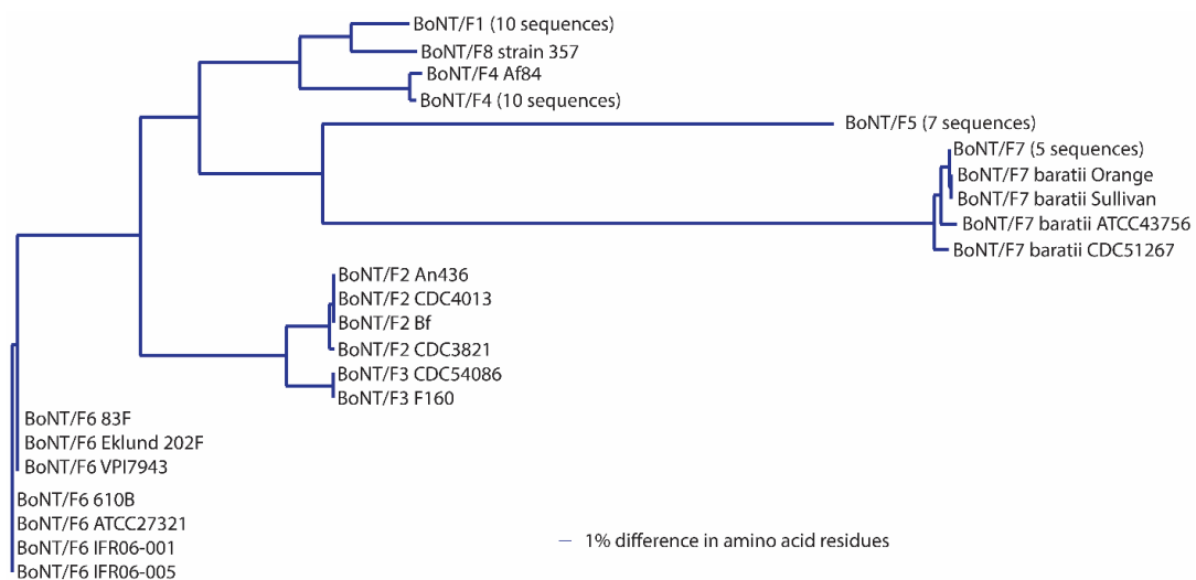
Figure 6. Dendrogram showing the relationships of BoNT/F subtypes. A total of 52 amino acid sequences were analyzed. The scale for this dendrogram is significantly smaller than with the others due to the wider range of identity differences (7.8%–36.2%) within this serotype.
