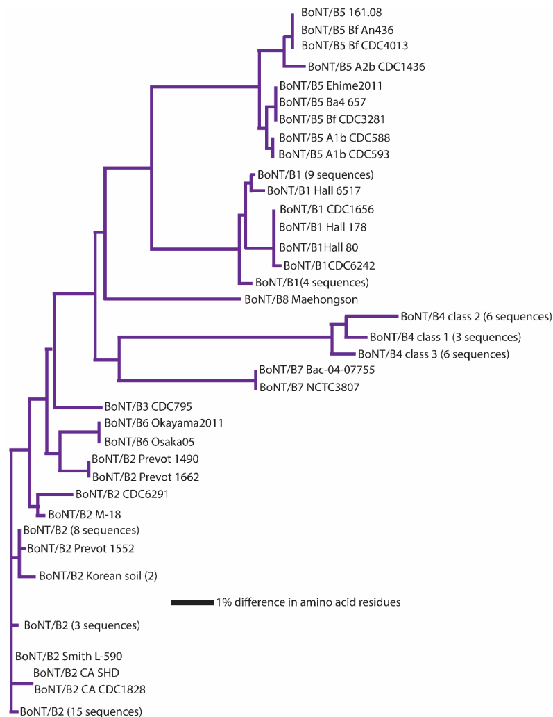
Figure 3. Dendrogram showing the relationships of BoNT/B subtypes. A total of 91 amino acid sequences were analyzed. The BoNT/B subtypes show the closest relationships, with amino acid differences ranging from 1.6%–7.1%.
