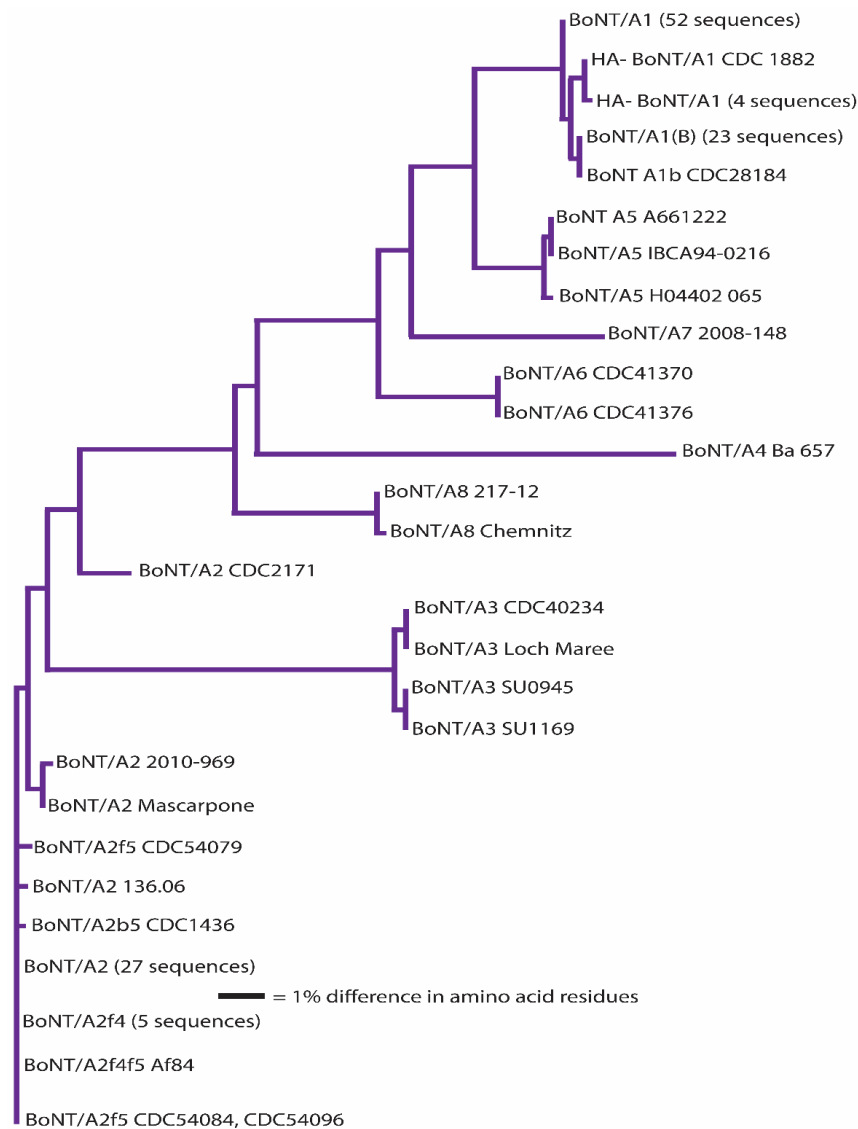
Figure 2. Dendrogram showing the relationships of BoNT/A subtypes. A total of 127 amino acid sequences were analyzed. “HA-” indicates BoNT/A1 encoding gene within a toxin cluster lacking genes encoding hemagglutinin proteins.
