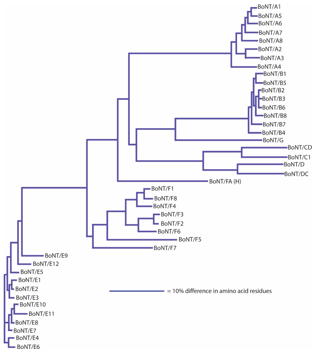
Figure 1. Dendrogram showing the relationship of all published/publicly-posted BoNT subtypes. The dendrograms were generated from protein sequence data using ClustalW with the representatives listed in Table 3. BoNT/FA is also known as BoNT/H and BoNT/HA (see the text for further details).
