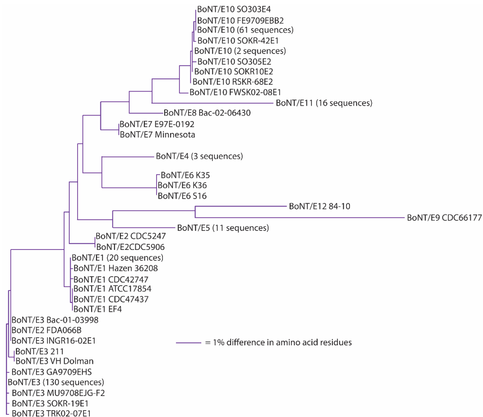
Figure 5. Dendrogram showing the relationships of BoNT/E subtypes. A total of 235 amino acid sequences were analyzed.
