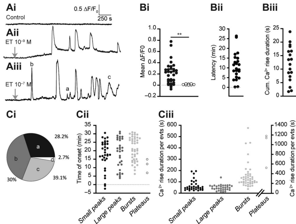
Fig. 5. ET induces intracellular [Ca^{2+}]_i rise in oligodendrocytes. Changes in [Ca^{2+}]_i were monitored by determining the relative changes in fluorescence ( \Delta F/F_0 ) of cells loaded by the Oregon green probe.
