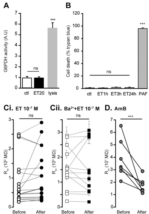
Fig. 4. ET does not induce membrane leakage, cell death or pore formation.
