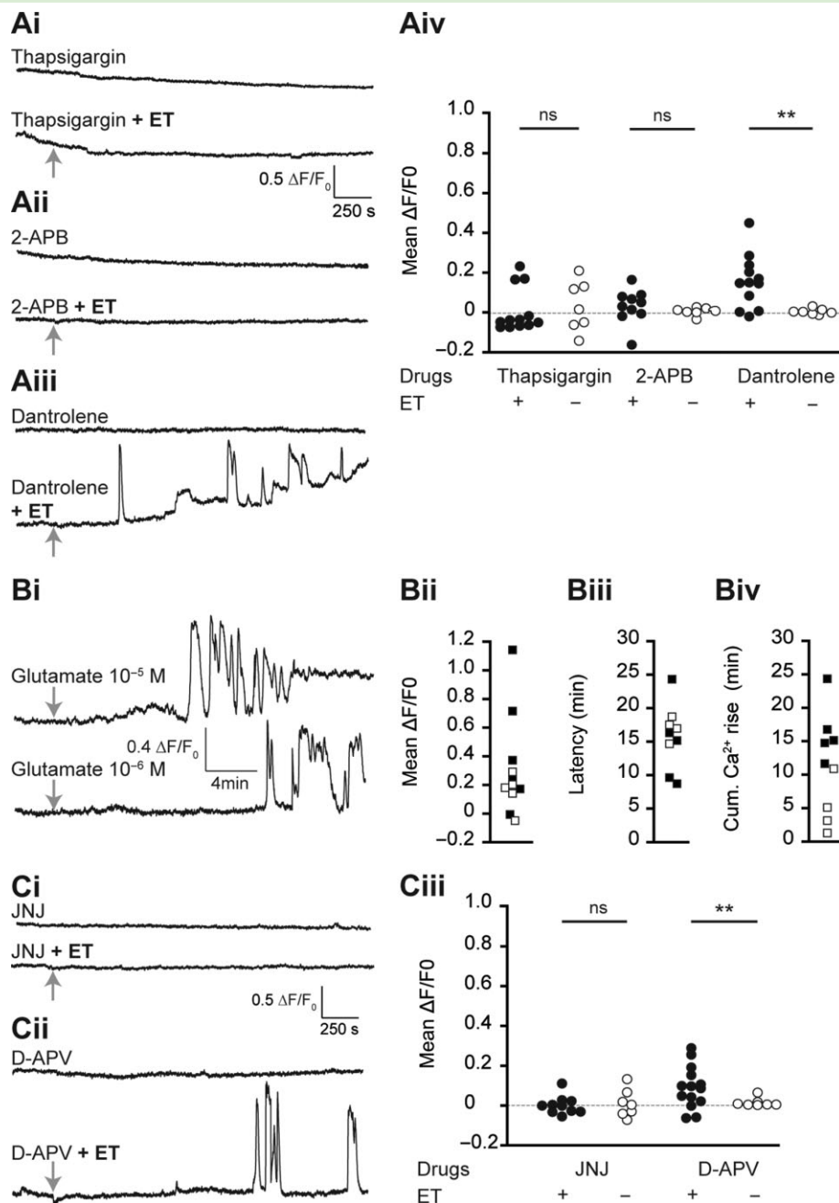
Fig. 6. Pharmacological dissection of ET-induced \text{Ca}^{2+} signalling pathway.
