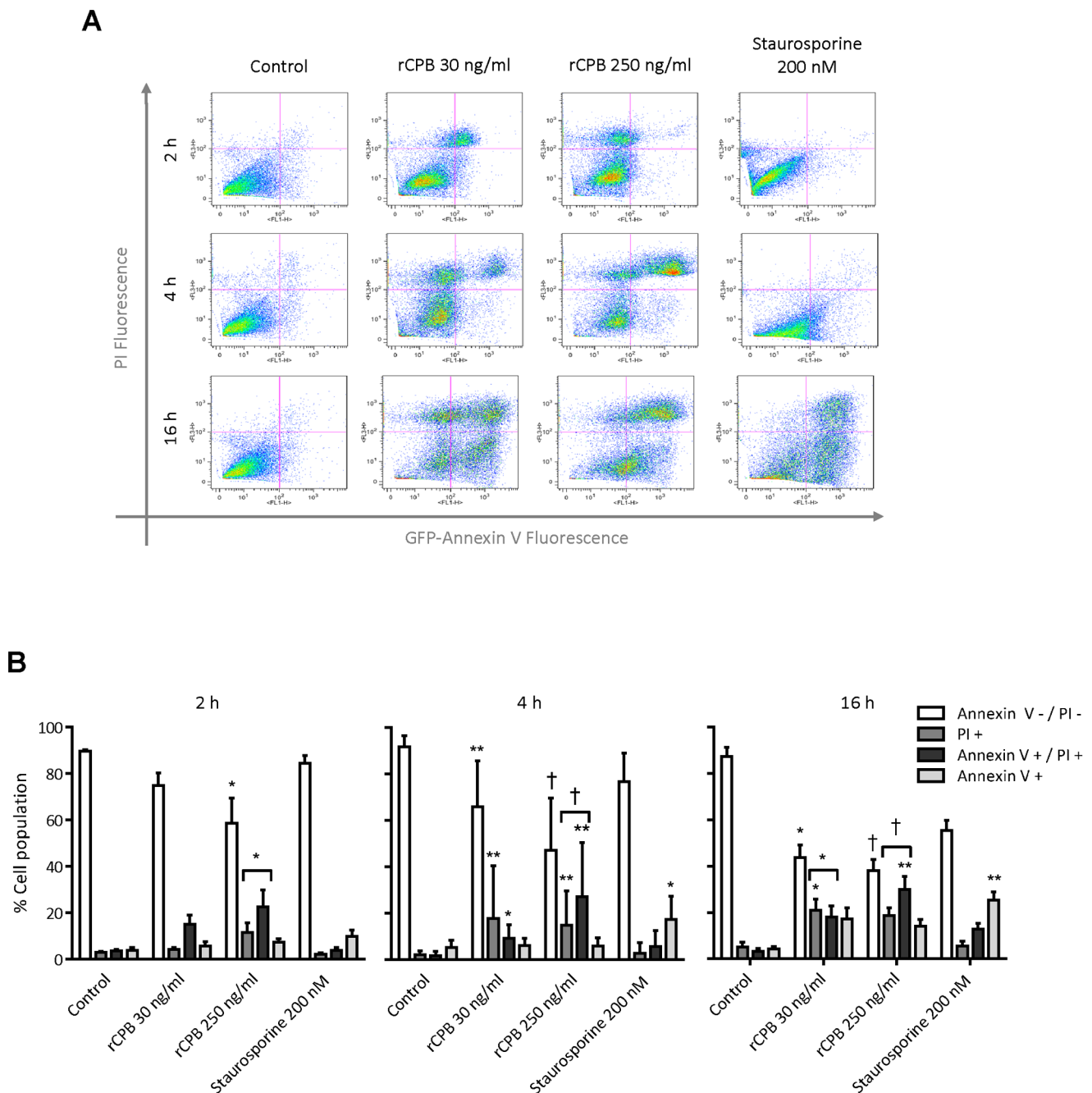
Figure 2. Characterization of rCBP-induced cell death by FACS analysis. pEC were either left untreated or exposed to 30 or 250 ng/ml of rCBP, or staurosporine, detached from the culture dishes by gentle trypsinization, and analyzed by FACS for PI uptake and GFP-annexin V staining at 2, 4 and 16 h of incubation. (A) Representative cytograms and bar graphs (B) in which cells in the lower left quadrant (PI/annexin V double-negative) were considered to be viable (white), cells in the upper left quadrant (PI single-positive) to be necrotic (gray), cells in the lower right quadrant (annexin V single-positive) to be apoptotic (light gray), and cells in the upper right quadrant (PI/annexin double-positive) to be either necrotic or secondary necrotic after apoptosis (dark gray). Bar graphs show quantitative summary of FACS analysis from 3 to 6 independent experiments. Results are expressed as mean \pm SD. Statistical difference to control cells was assessed by non-parametric Kruskal-Wallis and Dunn's post-hoc test. * P < 0.05 , ** P < 0.01 , † P < 0.001 .
