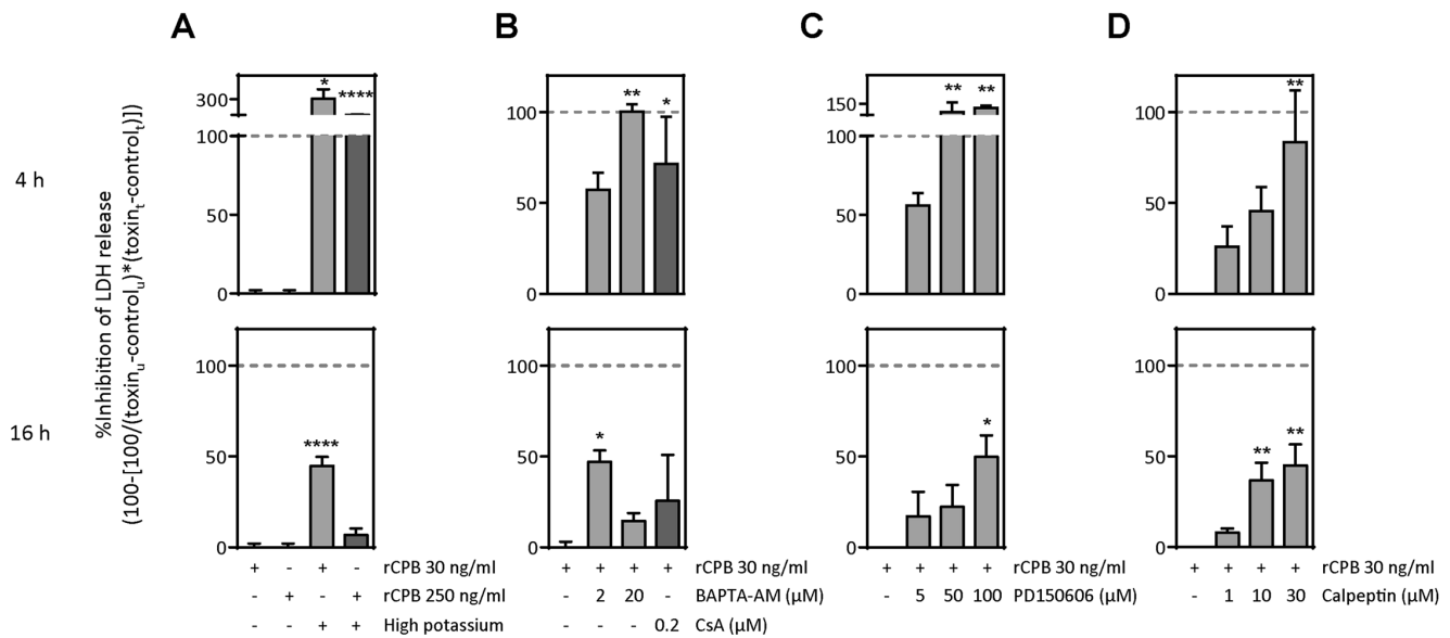
Figure 6. Attenuation of rCPB-induced necrosis by high extracellular K^+ , chelation of intracellular Ca^{2+} , and calpain inhibition. (A) Suppression of potassium efflux by high K^+ medium (140 mM) significantly inhibited rCPB-induced LDH release from pEC at 4 h, and still reduced LDH release at 16 h, when cells were exposed to 30 ng/ml rCPB. (B) Chelation of intracellular Ca^{2+} with BAPTA-AM (2 or 20 \mu M) or treatment with cyclosporin A (200 nM) markedly inhibited rCPB induced LDH release at 4 h, and to a lesser extent at 16 h post-exposure. LDH release of rCPB-treated cells in absence or presence of increasing concentrations of PD150606 (C) or calpeptin (D) was measured at 4 and 16 h. Bar graphs show summary of results from 2 to 5 independent experiments, which are expressed as percentage \pm SEM relative to rCPB-treated cells in the absence of inhibitor or presence of low K^+ medium (=control). Statistical difference to control was assessed by 1-way ANOVA and Dunnett post-hoc test. * P<0.05 , ** P<0.01 . u=untreated cells, t=treated cells. doi:10.1371/journal.pone.0064644.g006
