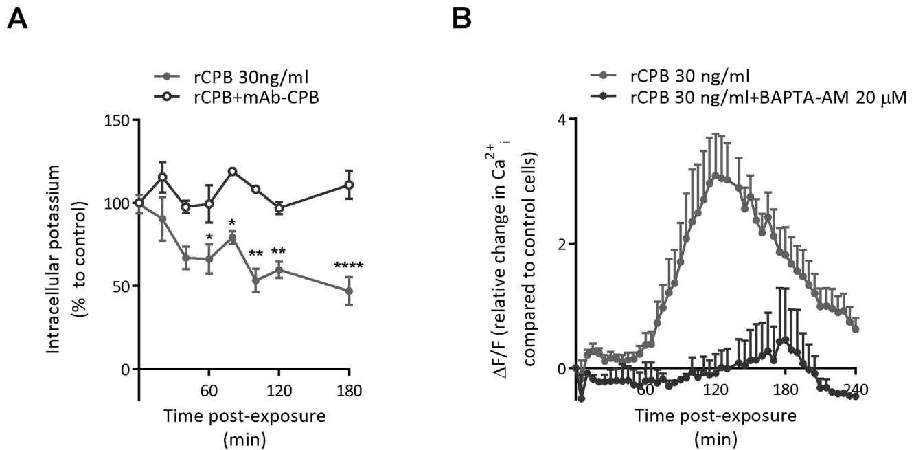
Figure 5. rCPB-induced efflux of K + and accumulation of intracellular Ca 2+ . (A) Incubation of confluent pEC with 30 ng/ml rCPB resulted in rapid and significant reduction of intracellular K + . rCPB preincubated with mAb-CPB did not cause K + efflux. Values represent means \pm SEM from 3 independent experiments. Statistical difference to cells treated with neutralized toxin (=control) was assessed by 2-way ANOVA and Bonferroni multiple comparisons test. *P<0.05, **P<0.01, ****P<0.0001. (B) Intracellular calcium ([Ca 2+ ] i ) levels were measured by Fluo-4 fluorescence in the presence of 3 mM extracellular CaCl 2 . Results are expressed as mean \pm SEM from 3 independent experiments. doi:10.1371/journal.pone.0064644.g005
