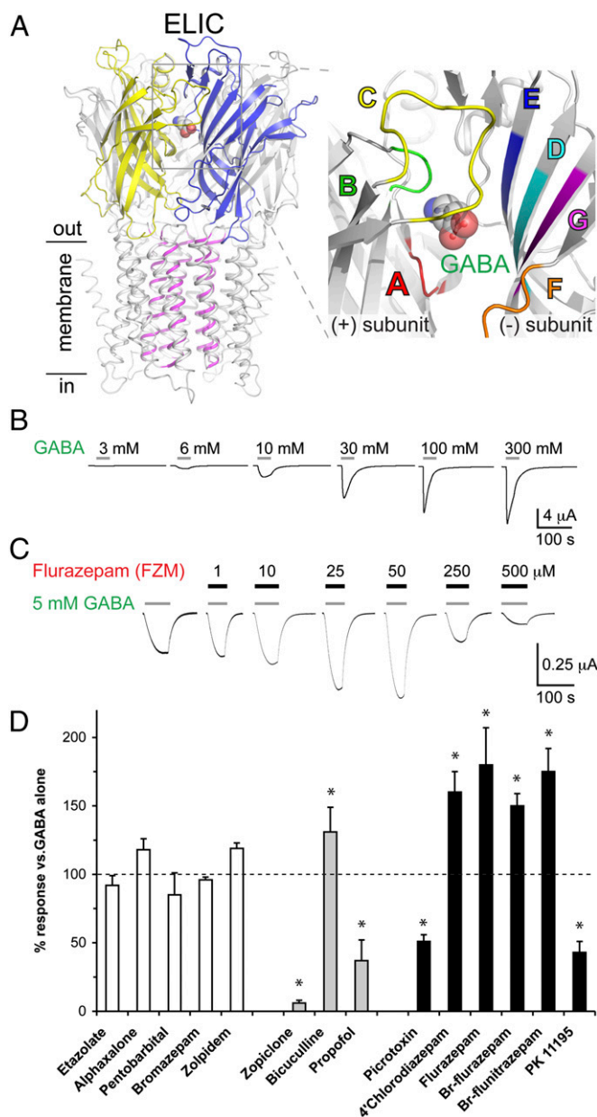
Fig. 1. ELIC is a bacterial GABA-gated channel, which is modulated by benzodiazepines. (A) (Left) X-ray crystal structure of ELIC in complex with GABA showing the location of the GABA-binding site between the principal (yellow) and complementary (blue) subunits. GABA is shown in spherical representation. (Right) Close-up view showing the different loops (A–G) that contribute to the ligand-binding site. (B) Typical traces of concentration-dependent GABA-induced current recorded from oocytes injected with ELIC. Horizontal bars indicate duration of agonist application. (C) Flurazepam (black bars) biphasically modulates the GABA-induced current. (D) Application of a range of GABA A -receptor modulators [10 \mu M each, except propofol (100 \mu M), etazololate (30 \mu M), alphaxalone (100 \mu M), pentobarbital (1 mM), flurazepam (50 \mu M), and PK11195 (100 \mu M)] to 3–5 mM GABA-induced ELIC currents shows that the effects of some GABA A -receptor modulators are conserved in ELIC. No modulators had effects when applied alone. Data are mean \pm SEM, n = 3 –5. * P < 0.05 .
