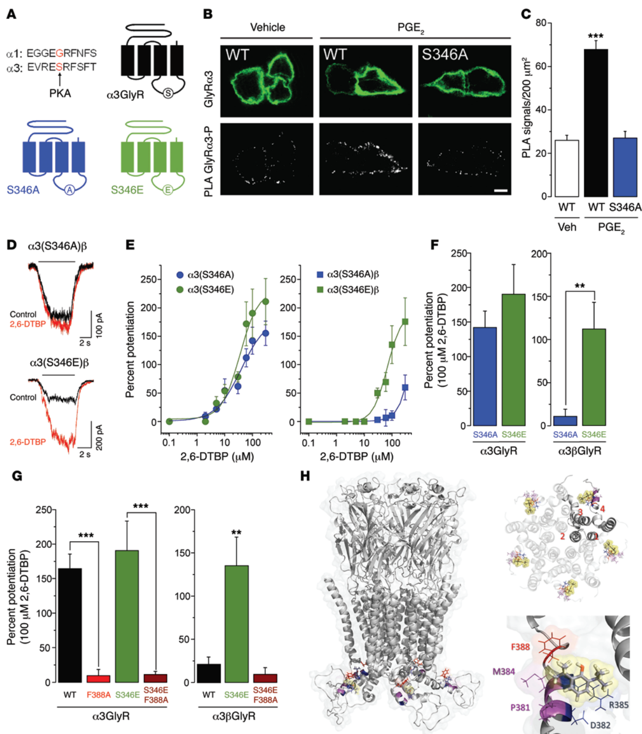
Figure 3. Influence of S346 phosphomutation in α3GlyR on allosteric modulation by 2,6-DTBP. (A) Localization of the S346 residue in the primary sequence of the mouse GlyR α3 subunit, the corresponding sequence in the GlyR α1 subunit, and schematic diagram illustrating this site in the α3GlyR topology. (B) Proximity ligation assay (PLA) demonstrating phosphorylation of α3GlyR by PGE 2 (1 μM) in HEK293T cells transfected with the EP2 receptor and wild-type GlyR α3 or (S346A) point-mutated GlyR α3 subunit plasmids. Top: α3GlyR immunofluorescence, bottom: PLA signal. Scale bar: 5 μm. (C) PGE 2 significantly increased PLA signals in HEK293T cells transfected with wild-type but not with (S346A) GlyR α3 subunits. *** P < 0.001, ANOVA followed by Bonferroni post-hoc test, F (2,141) = 49.84; P < 0.001, PGE 2 in wild-type α3GlyR-transfected cells versus the other two conditions. (D) Example traces of glycine-activated currents in α3(S346A)β or α3(S346E)βGlyRs in the absence and presence of 2,6-DTBP (100 μM). (E) Concentration-response curves for 2,6-DTBP in homomeric α3 (left) and heteromeric α3βGlyRs (right) containing S346E or S346A mutations. (F) The phosphomimicking S346E mutation restored 2,6-DTBP sensitivity of α3βGlyRs but had little effect on that of homomeric α3GlyRs. ** P < 0.01, unpaired t test. (G) The F388A point mutation in α3GlyRs abolished 2,6-DTBP sensitivity. Introducing the S346E mutation did not restore 2,6-DTBP sensitivity in homomeric α3(F388A)GlyRs or heteromeric α3(F388A)βGlyRs. ** P < 0.01, *** P < 0.001, ANOVA followed by Bonferroni post-hoc test, F (3,35) = 20.7 (left) and F (2,16) = 8.81 (right). (H) Structural model of the α3GlyR. Left: location of the F388 residue (red) and of 2,6-DTBP (yellow sphere) in a homopentameric α3GlyR. Other relevant residues are shown in magenta (P381 and M384) and blue (D382 and R385). Top, right: view from the middle of the plasma membrane on the putative acceptor sites with 2,6-DTBP bound (in yellow spheres) within a pentameric complex. Bottom, right: detailed view of the putative acceptor site of 2,6-DTBP. The hydrophobic interaction supported by F388 is highlighted in red.
