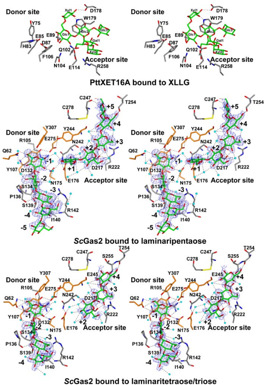
FIGURE 2. Structures of ScGas2-laminarioligosaccharide complexes. Stereo view of the active site of ScGas2 in complex with laminaripentaose and the hydrolysis products of laminariheptaose (i.e. laminaritetraose + laminaritriose), and comparison with PttXET16A bound to XLLG. The active site oriented to facilitate identification of the donor (left) and acceptor (right) subsites. The amino acids placed in the donor site and acceptor sites are shown as sticks with gray carbons. The residues targeted by site-directed mutagenesis, Gln 62 , Tyr 107 , Asp 132 , Asn 175 , Glu 176 , Tyr 244 , Glu 275 , Tyr 307 , Phe 404 , and Tyr 474 , are shown with orange carbon atoms. XLLG, laminaripentaose, laminaritetraose, and laminaritriose are represented as stick models with green carbon atoms. Protein-ligand and water-ligand hydrogen bonds are shown as dotted black lines. Water molecules involved in hydrogen bonds with the ligands are shown as cyan spheres. For clarity purposes, protein-water hydrogen bonds are not shown. Unbiased (i.e. before inclusion of any ligand model) |F_o| - |F_c| , \phi_{\text{calc}} electron density maps are shown at 2.5 \sigma .
