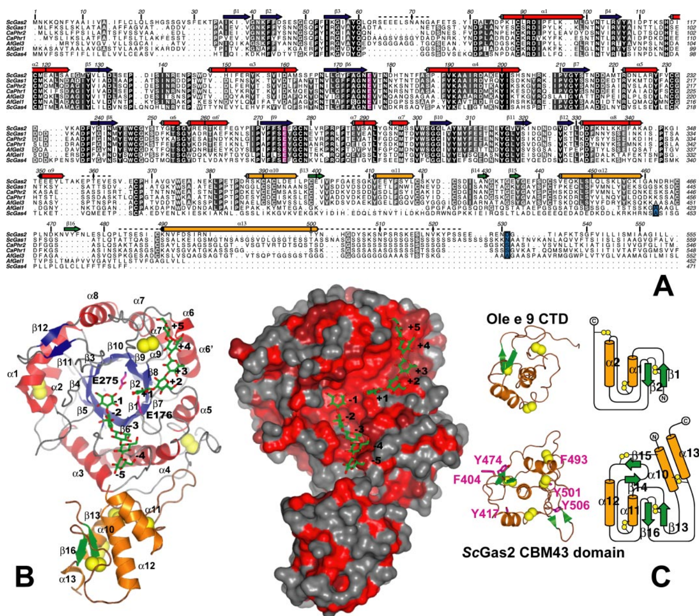
FIGURE 1. Overall structure of ScGas2 and comparison with structurally related proteins. A, multiple sequence alignment of the GH72 family members ScGas2, ScGas1, CaPhr2, CaPhr1, AfGel3, AfGel1, and ScGas4. Secondary structure elements from the ScGas2 structure are shown, with \alpha -helices in red and orange for the catalytic and cysteine-rich domains, respectively, and \beta -strands correspondingly in blue and green. Regions that are disordered in some or all of the ScGas2 structures are marked with a dashed line. Conserved catalytic glutamate residues are highlighted in pink boxing, and the (predicted) GPI-anchor attachment site is indicated in blue boxing. B, overall crystal structure of ScGas2 in complex with laminaripentaose. The Glu 176 and Glu 275 are shown with pink carbon atoms and labeled. The seven disulfide bridges are highlighted in yellow. Helix \alpha 13 was not built in the laminaripentaose complex structure and thus is absent from this figure. Ligand molecules are shown as sticks with green carbon atoms and the sugar-binding sites are labeled -5 to +5, following standard nomenclature. Other colors as in A. Also shown is a surface representation of the ScGas2, colored by sequence conservation (red (100% identity) to gray (<50% identity)). C, comparison of the CBM43 domains of ScGas2 (bottom; E176Q mutant) and Ole e 9 (top; PDB ID 2JON (39)). Disulfide bridge sulfur atoms are shown as yellow spheres. Secondary structure elements are colored as in B and labeled. Unique features of either structure are shown in lighter colors in the picture (left). The topology diagram was drawn with Topdraw (50). Surface-exposed aromatic amino acids of the CBM43 domain of ScGas2 (Phe 404 , Tyr 417 , Tyr 474 , Phe 493 , Tyr 501 , and Tyr 506 ) are shown as sticks with pink carbon atoms.
