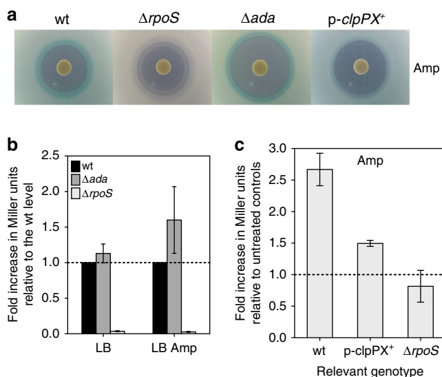
Figure 1 | Monitoring induction of the RpoS regulon using the pada::lacZ reporter fusion. Induction was visualized as blue rings using a disk diffusion assay on LB plates supplemented with X-gal (a) and by quantifying \beta -galactosidase activity in liquid LB medium (b,c). (b) Wild-type (wt), \Delta ada and \Delta rpoS strains grown in LB and LB supplemented with 1 \mu\text{g ml}^{-1} of ampicillin (Amp) (LB Amp). For each genotype, the fold increase relative to the wt level for each experimental condition is presented. (c) wt, wt strain overexpressing the ClpP–ClpX complex and the \Delta rpoS strain grown in LB supplemented with 1 \mu\text{g ml}^{-1} of ampicillin. For each genotype, the fold increase relative to the untreated control is presented. For all measures, each point represents the mean \pm s.e.m. of three independent experiments.
