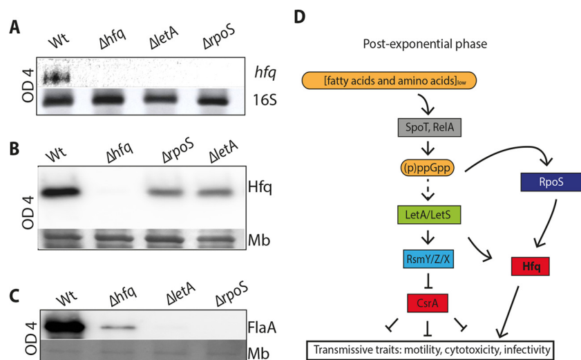
FIG 4 hfq transcript and protein expression are influenced by LetA and RpoS and impact flagellar expression. (A) Northern blot analyses of hfq transcripts in wt L. pneumophila and the \Delta hfq , \Delta letA , and \Delta rpoS regulatory mutants grown until they reached an OD 600 of 4 show that the hfq transcript is under the control of LetA and RpoS and is abolished in the \Delta hfq mutant. (B) Western blot analysis of Hfq protein levels in wt L. pneumophila and \Delta hfq , \Delta letA , and \Delta rpoS mutants grown until an OD 600 of 4 revealed a significantly decreased expression of Hfq in the regulatory mutants, indicating that RpoS and LetA influence Hfq expression. (C) Western blot analysis of FlaA protein levels in wt L. pneumophila and \Delta hfq , \Delta letA , and \Delta rpoS mutants grown until an OD 600 of 4 revealed that expression of FlaA is strongly decreased in the \Delta hfq mutant and as expected missing in the \Delta letA and \Delta rpoS mutants, suggesting that Hfq also influences flagellar expression. Mb, stained membrane signal as a loading control. (D) Schematic overview of the major regulatory elements governing L. pneumophila virulence expression in transmissive/postexponential phase and the place and role of Hfq in this network.
