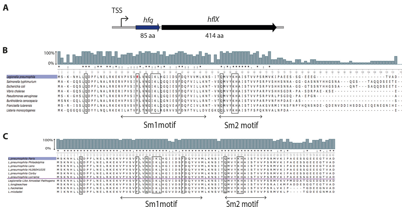
FIG 1 Legionella Hfq is conserved across the genus and other bacterial species. (A) Schematic organization of the L. pneumophila hfq locus. TSS, transcription start site; aa, amino acids. (B) Alignment of the L. pneumophila Hfq protein sequence with other bacterial Hfq protein sequences reveals high sequence and RNA binding site conservation. (C) Alignment of the L. pneumophila Paris Hfq protein sequence with the Hfq protein sequences from different L. pneumophila strains and other Legionella or Legionella -like species. Amino acids involved in RNA binding are boxed. Conserved amino acid residues (asterisks) and semiconservative substitutions (dots) and conservative substitutions (colons) are indicated. The bars above the sequence alignment indicate the sequence percentage of sequence conservation.
