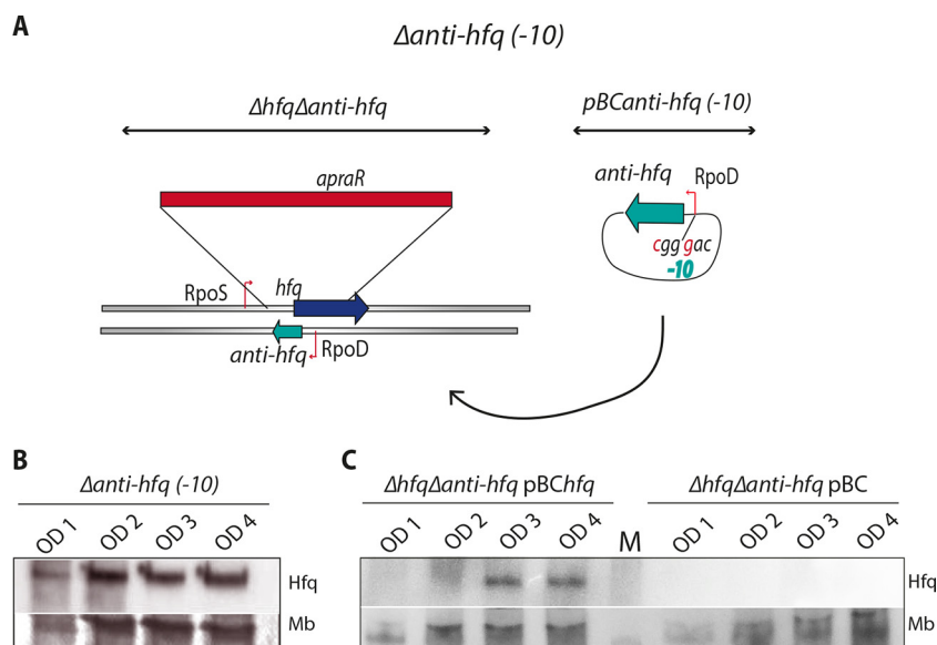
FIG 6 In an anti-hfq mutant, Hfq is already expressed during exponential growth. (A) Schematic presentation of the \Delta hfq \Delta anti\text{-}hfq mutant and sequence changes introduced in the anti-hfq promoter region to construct the \Delta anti\text{-}hfq(-10) mutant without disrupting the Hfq amino acid sequence. (B) The Anti-hfq sRNA influences Hfq protein expression as evaluated by Western blot analysis of Hfq in the \Delta anti\text{-}hfq(-10) mutant strain. Stained membrane (Mb) signals are shown as a loading control. (C) Western blot analysis of Hfq protein levels in the \Delta hfq \Delta anti\text{-}hfq mutant complemented with hfq and anti-hfq ( \Delta hfq \Delta anti\text{-}hfq pBChfq) shows that the growth phase-dependent Hfq expression pattern is restored. In contrast, the control strain carrying the empty plasmid ( \Delta hfq \Delta anti\text{-}hfq pBC) does not express Hfq. Stained membrane (Mb) signals are shown as loading control. M, molecular weight marker.
