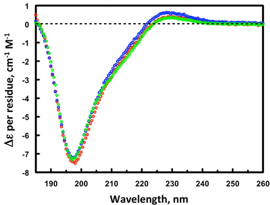
Figure 5. Circular dichroism of F19ec,ri, F19bac,r and F19bac. Superimposition of the circular dichroism far-UV spectra of F19ec,ri (red), F19bac,r (blue) and F19bac (green). doi:10.1371/journal.pone.0057086.g005
