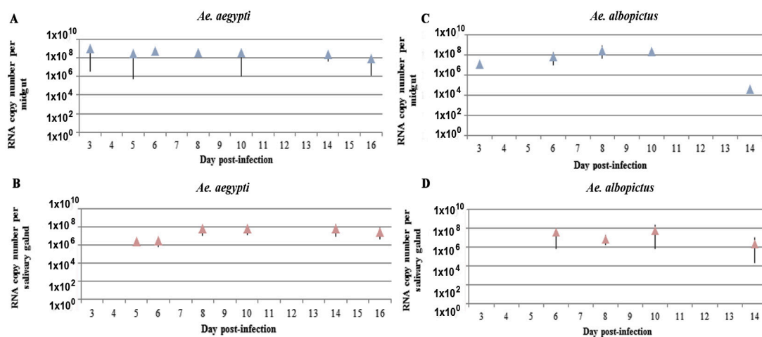
Figure 4. Kinetics of ZIKV infection of MG and SG of Ae. aegypti and Ae. albopictus measured by RT-qPCR. MG (A,C) and SG (B,D) infected by ZIKV in Ae. aegypti (A,B) and Ae. albopictus (C,D). Mean (triangles) and standard deviation (vertical bar) are presented for each organ in both species. Five to ten mosquitoes were sampled for each time.
