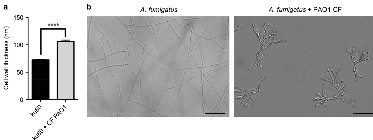
Figure 4 A. fumigatus hyphal morphology grown in presence of 24 h PAO1 CF. (a) Thickness of A. fumigatus ku80 cell wall in presence of CF in RPMI, calculated from 50 hyphae with six measures per hyphae from TEM pictures using the ImageJ/fiji analysis (Schneider et al, 2012). (b) Light microscopy images showing the increased branching of the fungal hyphae in presence of CF. Scale bar 50 \mu m.
