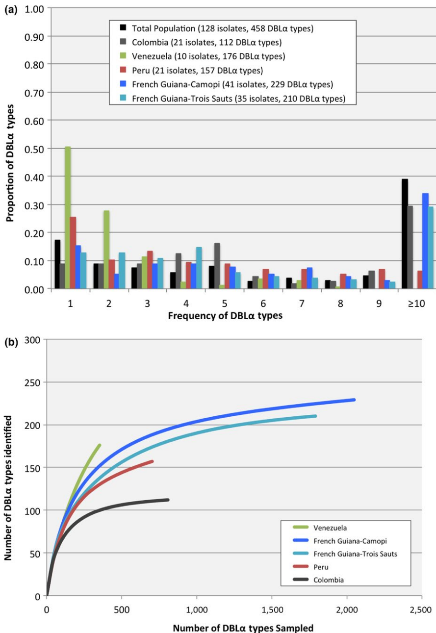
FIGURE 2 Frequency distribution and diversity of var DBLα types in the population. (a) For the South American isolates, clustering of the 5,699 DBLα sequences resulted in 458 unique var DBLα types. The figure provides the proportion of var DBLα types that appeared one to ten or more times within and among all the South American populations. (b) Cumulative diversity curves for the var DBLα types sampled in each South American population. The Venezuelan curve (green) does not show evidence of leveling off, in contrast to those for Colombia (grey), Peru (red), French Guiana-Camopi (blue) and French Guiana-Trois Sauts (turquoise). The up-sloping curve for Venezuela suggests that more DBLα types will be found with further sampling of this population
