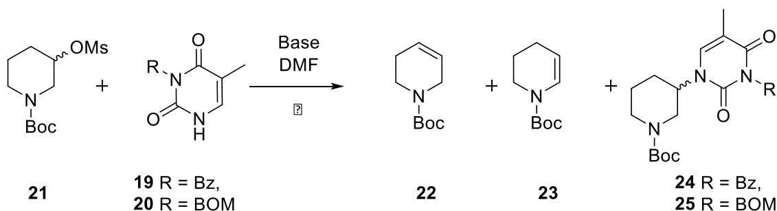
Scheme 2: Alkylation of N3-protected thymine using piperidinylmesylates
