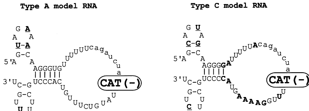
Fig. 1. Nucleotide sequences and predicted (Flick et al. , 1996) hairpin loop structures of the model RNA templates. The nucleotide sequences of the type A and C model RNAs transcribed from plasmids pA/PRCAT and pC/PRCAT are those of the NS genome segment (uppercase) of the A/WSN/33 and C/JHB/1/66 strains of influenza virus. Nucleotides shown in bold differ between the type A and C model RNAs. The nucleotides studied in this paper are underlined. Unrelated nonviral sequences are shown in lowercase.
