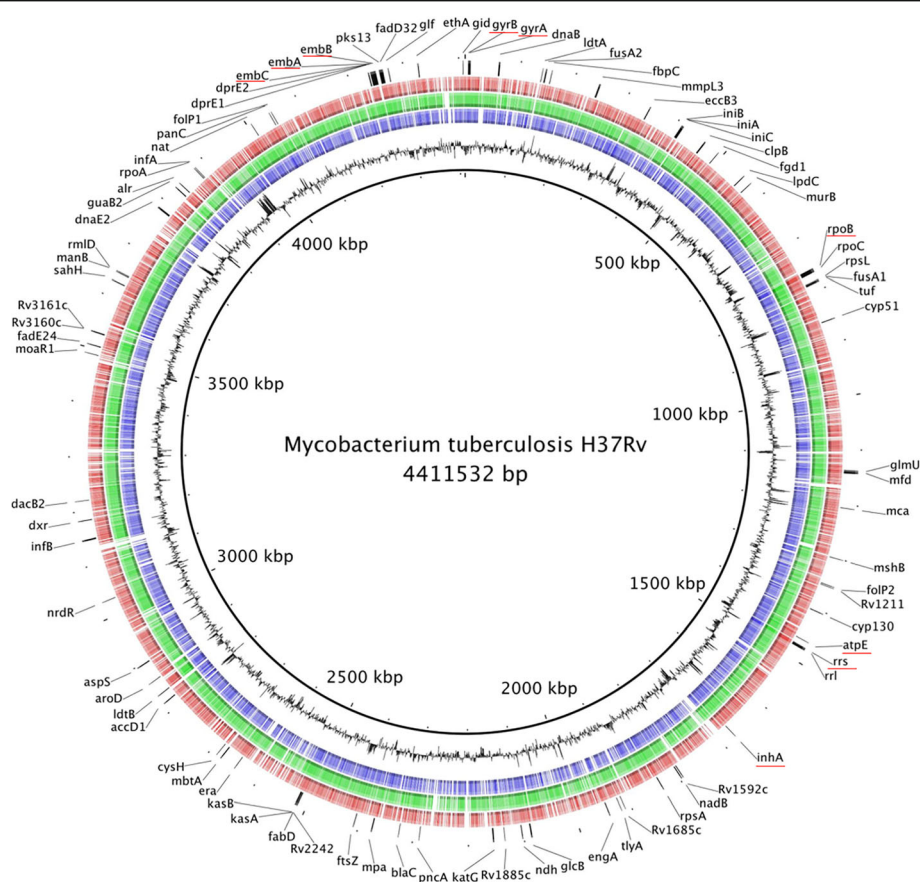
Fig. 3 Whole genome alignment of the model species relative to M. tuberculosis . Each ring corresponds to one genome. Blue ring, M. marinum ; Green ring, M. smegmatis ; red ring, M. aurum . The indicated genes correspond to those that are already reported to be associated with mycobacterium drug resistance
