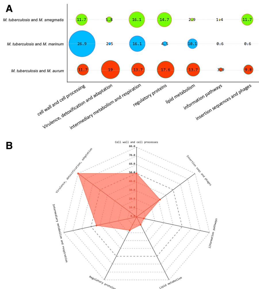
Fig. 4 Shared metabolic pathways based on the specific identified genes between the surrogate model species and M. tuberculosis H37Rv. a dot plot showing the data corresponding to Tuberculist functional categories of the genes that are specific to each model species relative to M. tuberculosis , strain H37Rv. The number inside each circle represent the proportion of each category. b radar chart showing the number of each genes in each Tuberculist functional category relative to the 419 specific genes to Mycobacterium tuberculosis , strain H37Rv. For graphical convenience, in both (a) and (b) graphs, the data relative to genes coding for unknown functions are not shown. For more details refer to Additional files 1, 2, 3, 4, 5, and 6
