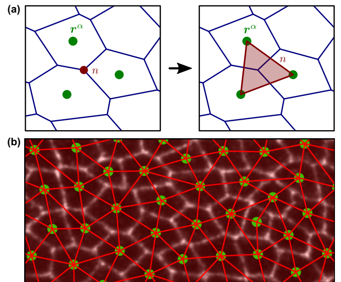
FIG. 2. Triangulation of the cellular network. (a) Each threefold vertex n (red dot) gives rise to a single triangle (red), which is also denoted by n . The corners of the triangle are defined by the centers of the three abutting cells (green dots). (b) Triangulation (red) on top of membrane-stained biological tissue (white). There are no gaps between the triangles.
