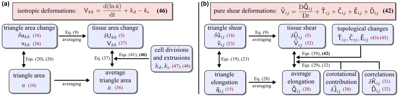
FIG. 13. Decomposition of deformations in cellular contributions. Key quantities and their relationships are shown as a schematic diagram. (a) Decomposition of the isotropic deformation rate into cellular contributions. (b) Decomposition of the pure shear rate into cellular contributions. Red numbers indicate the definition of the respective quantity (or the equation where the quantity first appears). Black numbers indicate important relations between the quantities.
