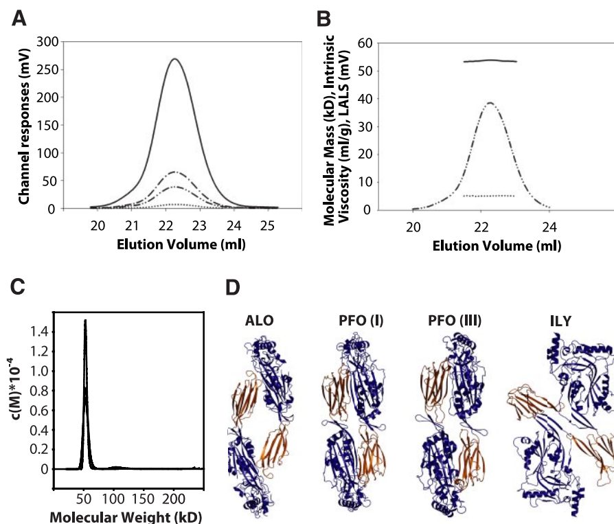
FIGURE 4. Oligomerization analysis and hypothetical dimer configurations. A, chromatograms of ALO from S200 size exclusion chromatography coupled to differential pressure transducers and SLS and UV detectors. Data lines show UV (solid), RALS (dot-dash), LALS (dot-dot-dash), and DP (dotted). B, molecular weight (MW) and intrinsic viscosity (IV) patterns of ALO. Data lines show molecular weight (solid), LALS (dot-dot-dash), and IV (dotted). The retention volume of ALO (22.2 ml) is probably due to interactions with the column media. Using standard proteins for calibration, such a retention volume corresponds to a 15–20-kDa protein (not shown). Hence, measurement of molecular mass by SEC-SLS, which is independent from the retention volume on SEC, is appropriate for ALO. C, sedimentation velocity analysis of ALO from analytical ultracentrifugation at three different pH values: pH 5.5 (dashed), pH 7.0 (solid), and pH 8.0 (dotted). D, potential dimer interactions. Crystallographic dimers are found in ALO and PFO (I) crystals, and noncrystallographic dimers are seen in PFO (III) and ILY crystals. Domains 1–3 are colored blue, and D4 is colored orange.
