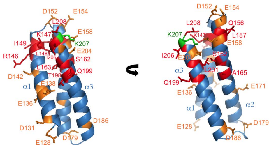
Supplementary Figure S8: a) Chemical shift perturbations of the observed ^1\text{H} (top) and ^{15}\text{N} nuclei (bottom) in Fap1-NR _{\alpha} at 950 MHz. Differences between pH 8 and pH 6 are shown in black bars and between pH 8 and pH 5 in grey bars. Bar are absent if the resonance was not assigned. Acidic residues in the sequence are annotated in orange while the other residues significantly affected are highlighted in red. The secondary structure of the helical bundle is shown above. B) Ribbon representation of the NMR structure of Fap1-NR _{\alpha} at pH 8. As reported in the histograms, side-chains of acidic residues are shown in orange. Residues displaying significant pH-induced chemical shift changes are indicated in red. K207 in the proximity of E158 and E204 is shown in green.
