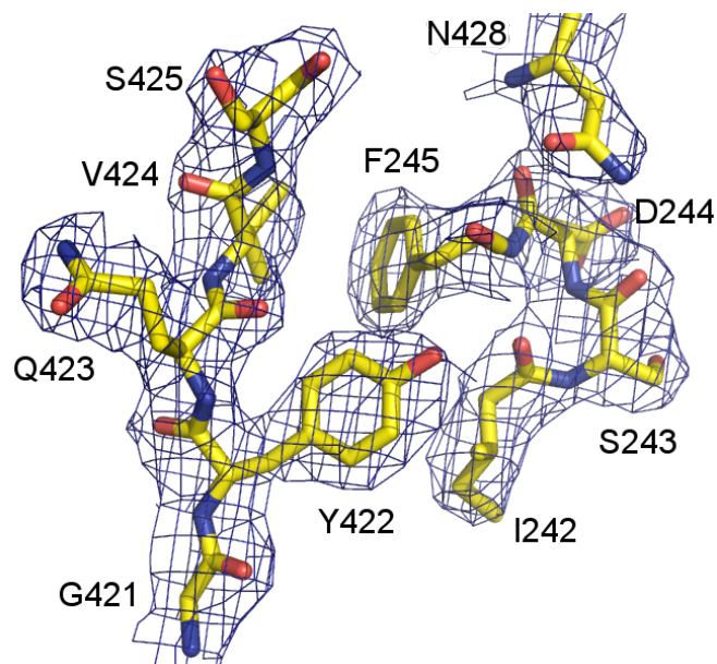
Supplementary Figure S1: An example of the electron density quality of the Fap1-NR \beta structure. Residues 242-245, 421-425 and 428 of chain A are shown as sticks with sigma A weighted maps contoured at 1 r.m.s electron density.
