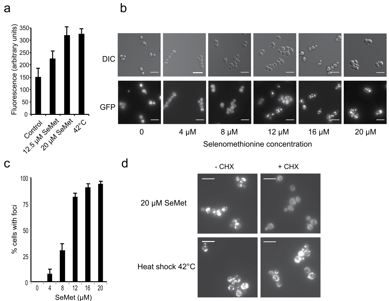
Figure 2. SeMet promotes protein aggregation in vivo . (a) Induction of Hsp104-GFP by SeMet or heat shock. Exponentially growing BY4741-Hsp104-GFP cells were incubated in SC + 100 \mu\text{M} methionine for 2 h, either at 30 °C in the presence of the indicated concentration of SeMet or at 42 °C in the absence of SeMet. The fluorescence in whole cell extracts was recorded at 508 nm and normalized to the optical density of the extracts at 280 nm. The fluorescence of an extract from untagged BY4741 strain grown in SC + 100 \mu\text{M} methionine was subtracted from the results. The results are the mean \pm S. D. of at least 3 experiments. (b) Hsp104-GFP localization was monitored by fluorescence microscopy (GFP) and differential interference contrast (DIC), in living BY4741-Hsp104-GFP cells after 1 h of exposure to various SeMet concentrations in SC + 100 \mu\text{M} methionine. Representative images obtained after maximum intensity z-projection, bar equals 10 \mu\text{m} . (c) Quantification of protein aggregation. The fraction of cells containing at least one Hsp104-GFP focus was determined by visual inspection of 300–600 cells in each condition. The results are the mean and range of at least 2 experiments. (d) Effect of cycloheximide (CHX) on protein aggregation induced by 1 h of exposure to 20 \mu\text{M} SeMet or heat shock at 42 °C. BY4741-Hsp104-GFP cells grown in SC + 100 \mu\text{M} methionine were treated or not with 5 \mu\text{g}/\text{ml} cycloheximide for 1 h prior to the SeMet or heat-shock stress. Hsp104-GFP localization was monitored in living cells by fluorescence microscopy. Representative images obtained after maximum intensity z-projection, bar equals 10 \mu\text{m} .
