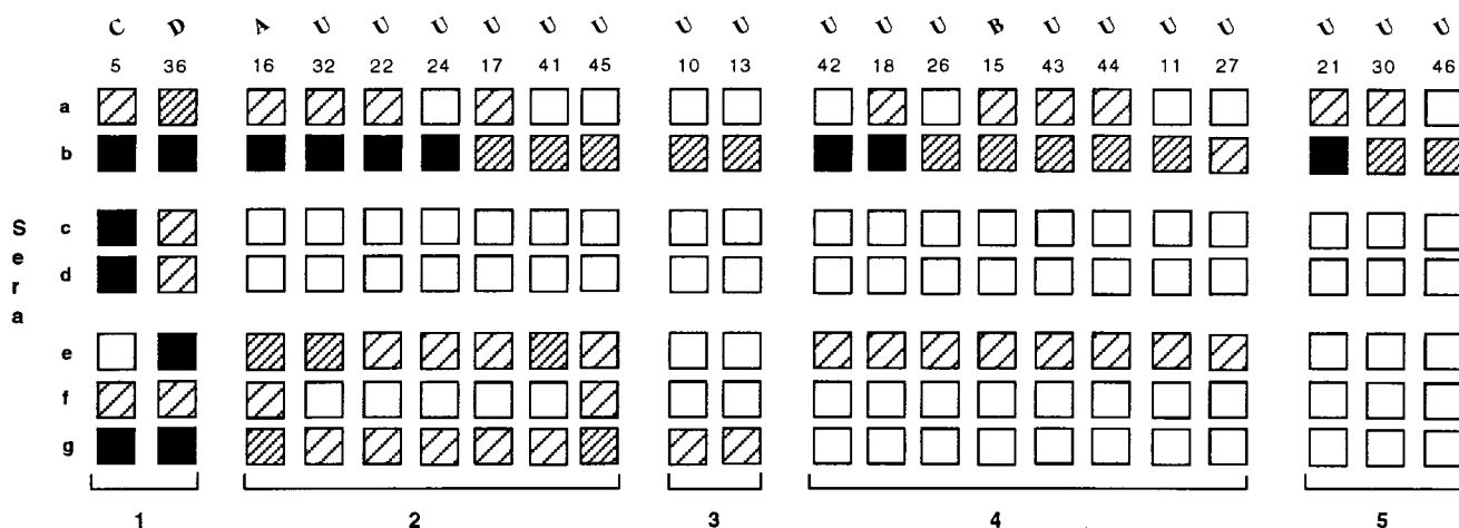
FIG. 2. Summary of the immunological reactivities of 22 representative clones (one from each hybridization cluster and the 18 single clones), reacted by using the plaque immunoassay with various sera: Saimiri anti-O and anti-R reagents used to screen the library (a and b, respectively), the HIS pool of human hyperimmune antisera from Senegalese adults (c), the HIG_1 pool of immune human IgG (d), RIS, a rabbit serum raised to the membrane fraction of FUP/CP-infected human erythrocytes (e), and antibodies eluted from the surfaces of O- or R-infected Saimiri erythrocytes (f and g, respectively). A reactivity score was established for each plaque immunoassay; the scores used ranged from 4 (very strong) to 1 (marginal or no reactivity) (■, ▨, ▧, and □, respectively). Clones were classified in five groups, depending on their reaction with the human hyperimmune reagents (HIS and HIG_1 ), the RIS sera, and the surface-eluted antibodies. The hybridization cluster or group for each clone is indicated above the clone number.
