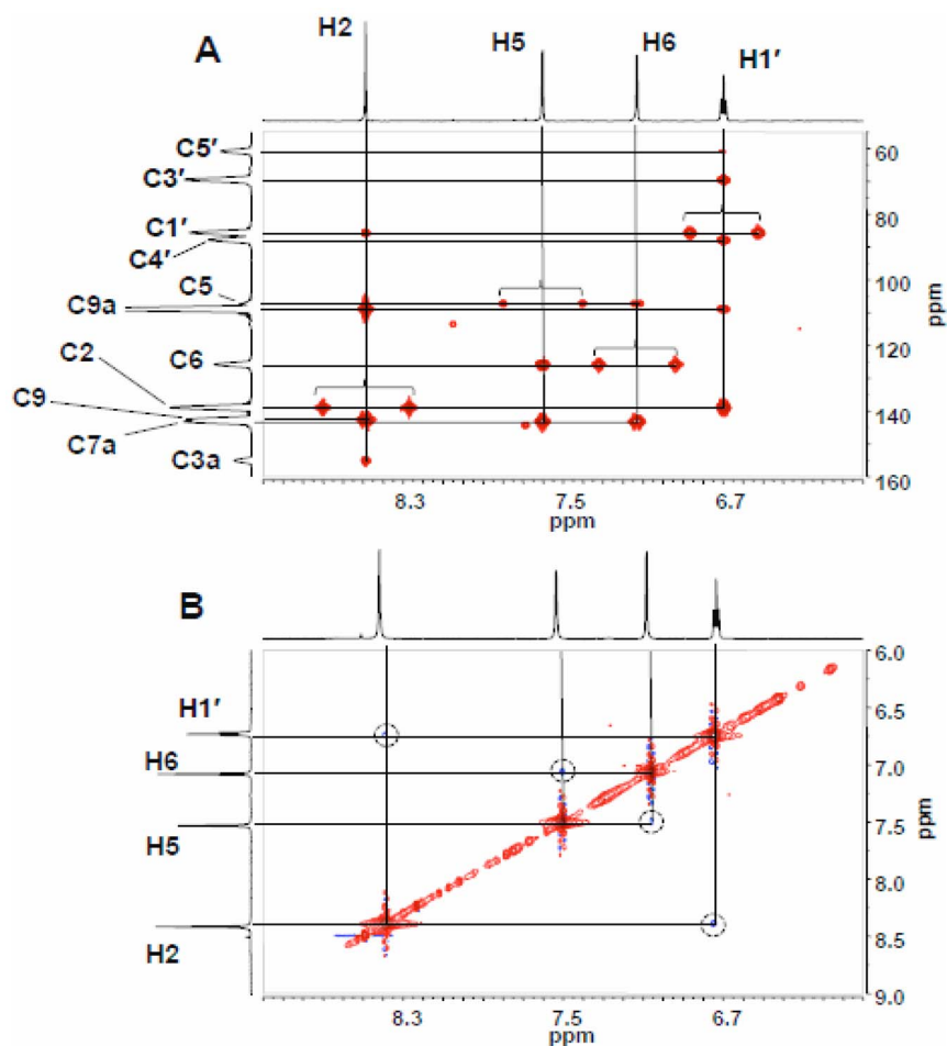
Fig. 6. Expansions of the HMBC (A) and NOESY (B) NMR spectra (DMSO- d_6 ) of the 16 min-eluting product of enzymatic ribosylation of 1 , spanning the region of H1'-etheno interactions. Proton signals are identified on the marginal spectral traces. In the HMBC spectrum, unsuppressed one-bond C-H couplings are indicated by brackets.
