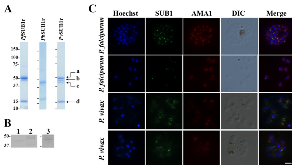
FIGURE 1. Expression of PbSUB1r , PfSUB1r , and PvSUB1r and characterization of endogenous PvSUB1 . A , Coomassie Blue staining of SDS-polyacrylamide gels of PbSUB1r , PfSUB1r , and PvSUB1r . Proteins were produced in baculovirus-infected insect cells, HPLC-purified, and concentrated (see “Experimental Procedures”). B , immunoblot of uninfected human erythrocytes (lane 1), P. falciparum 3D7 segmented schizonts (lane 2), and in vitro maturated P. vivax segmented schizonts (lane 3) probed with an anti- PvSUB1r serum. Molecular mass markers are in kDa. C , indirect immunofluorescence assays on air-dried P. falciparum 3D7 segmented schizonts (1st row of panels), individual merozoites (2nd row of panels), and P. vivax segmented schizonts (3rd and 4th rows of panels), probed with the anti- PvSUB1 polyclonal serum (green) and the anti-AMA1 rat monoclonal antibody 28G2 (red). Merozoite nuclei are labeled with Hoechst 33342. The scale bar represents 3 \mu\text{m} .
