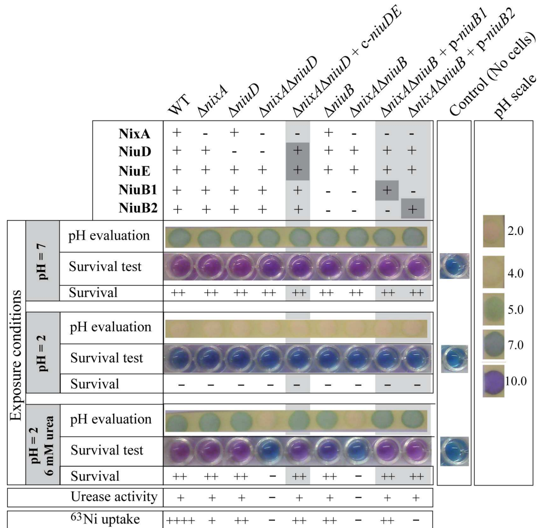
Fig 5. NixA and NiuBDE are necessary for resistance to extreme acidity in the presence of urea. Wild type strains and mutants were exposed during 40 min at pH 2, without or with 6 mM urea. \Delta niuB corresponds to a \Delta niuB1 - \Delta niuB2 double mutant. Controls were performed at pH 7 without urea. Survival of the bacteria was assessed using an Alamar blue-based test, in which a pink staining reveals metabolically active cells, while a blue staining means that cells are metabolically inactive. The pink staining is proportional to the amount of metabolically active cells. The pH was evaluated for each strain and results were compared to control cells (exposed at pH 7) and to a pH-scale (right side of the figure). A reminder of the results obtained in other experiments for urease activity and 63 Ni(II) uptake is given at the bottom of the figure for comparison.
