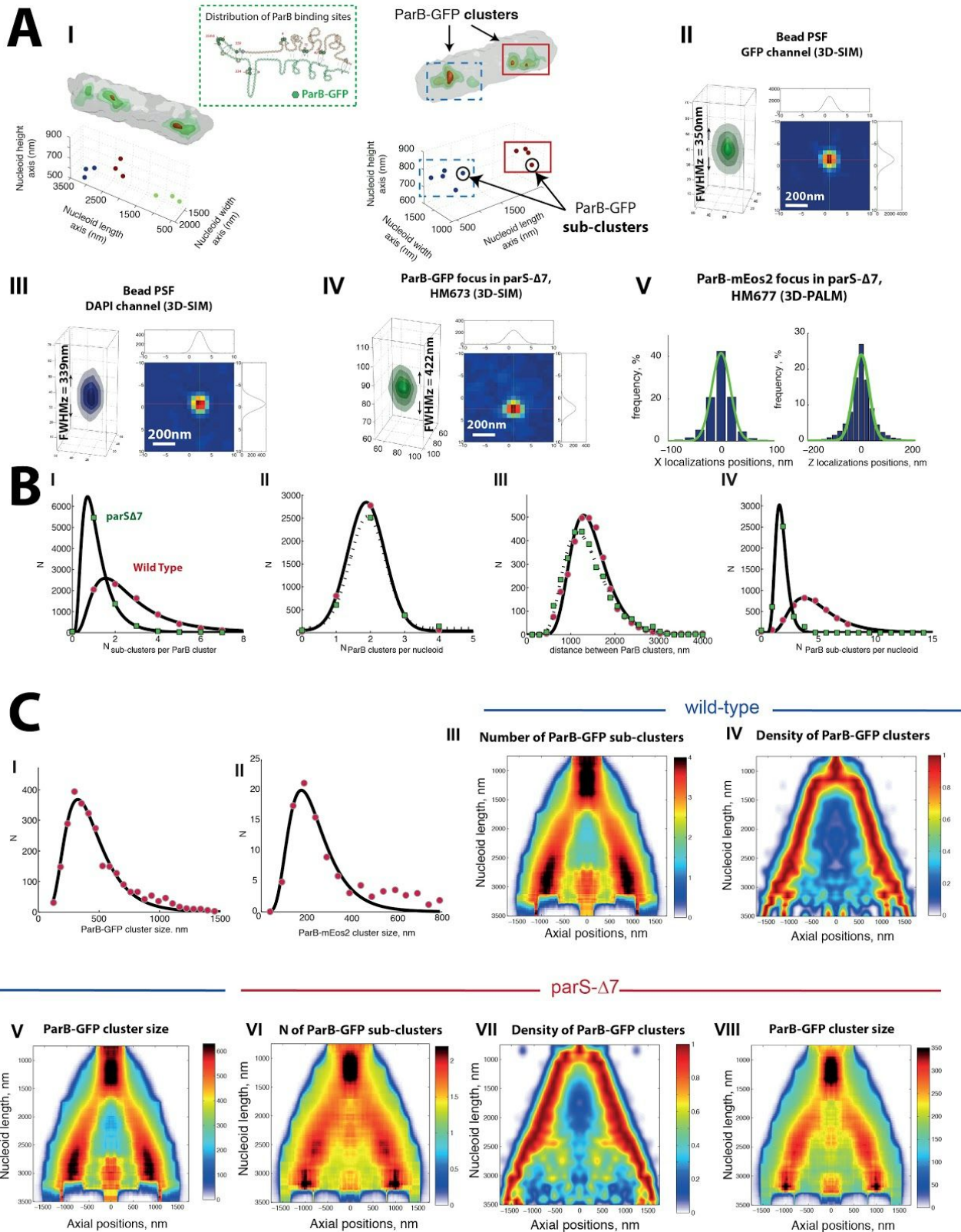
Figure S6. Analysis of origin domain dynamics probed by ParB-GFP, related to Fig. 6.
