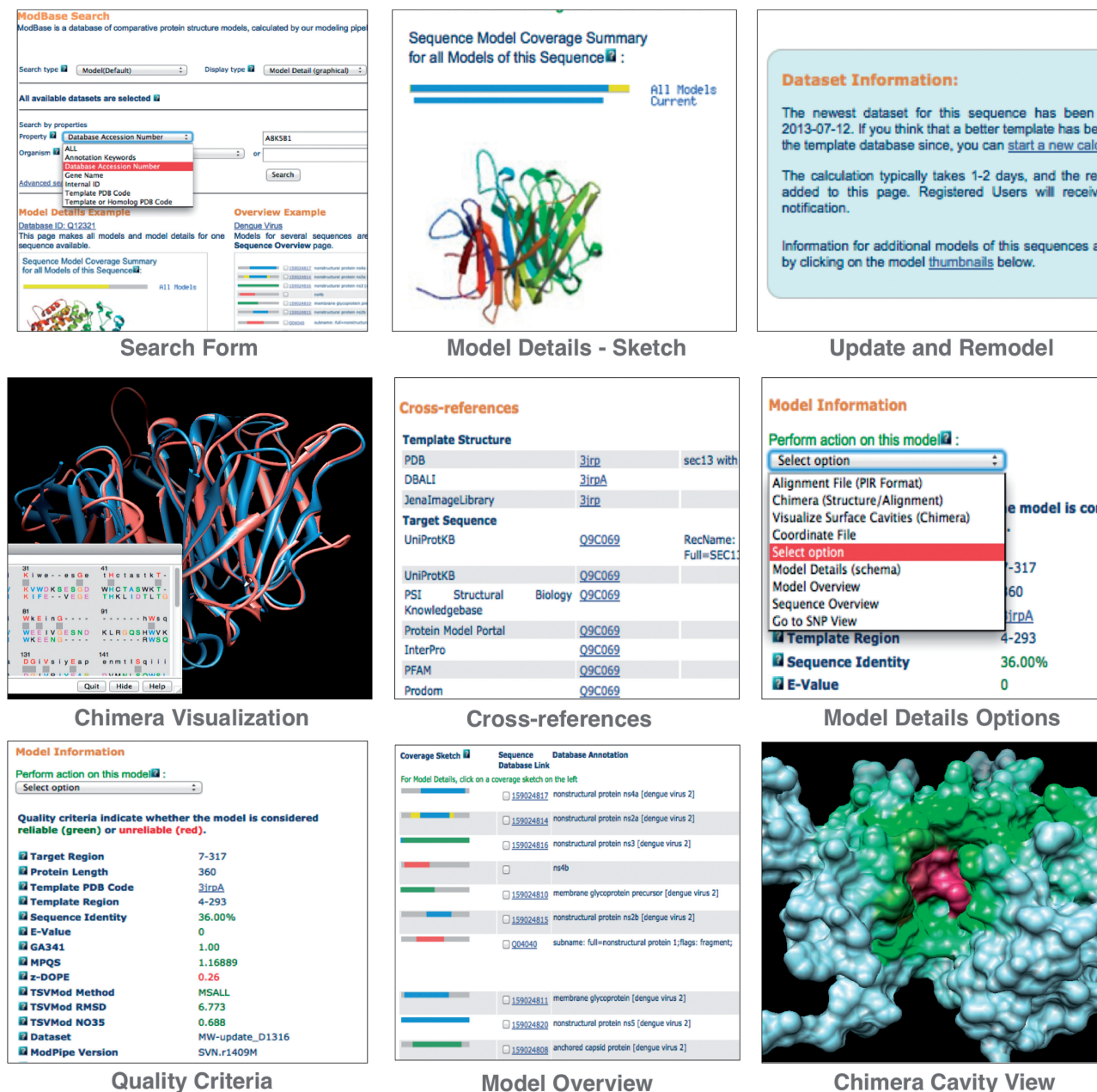
Figure 3. ModBase interface elements. Search Form: search options are available through the pull-down menu. A quick overview of the available representations is displayed below the search form. Model Details Sketch: the model details page provides information for all models of a given sequence. The sketch comprises two parts: the model coverage sketch that indicates the sequence coverage by all models (top line) and the sequence coverage by the current model (second line), and a ribbon diagram of the current model. Other models are available via thumbprints. Update and Remodel: this box shows the date of the last modeling calculation for the current sequence, and allows the user to request an update. Chimera Visualization: the visualization includes the model and template structures and the alignment. Cross-references: links to the PMP, UniProtKB, Genbank, UCSC Genome Browser and other databases. Model Details Options: the pull-down menu switches between representations and allows downloads of coordinate and alignment files. Quality Criteria: red indicates unreliable, green reliable. Model Overview: a different representation for several sequences gives a quick overview on modeling coverage and quality. Chimera Cavity View: visualizes cavities predicted by ConCavity.
