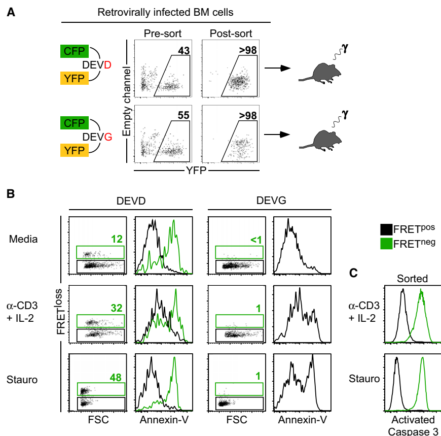
Figure 1. A Genetically-Encoded Reporter for Caspase-3 Activity Accurately Identifies Apoptotic T Cells
