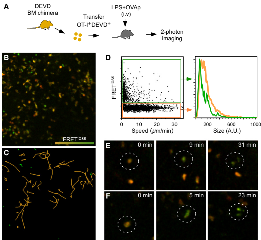
Figure 2. Caspase-3 Activity in T Cells Is Associated with Loss of Motility and Cell Death In Vivo
