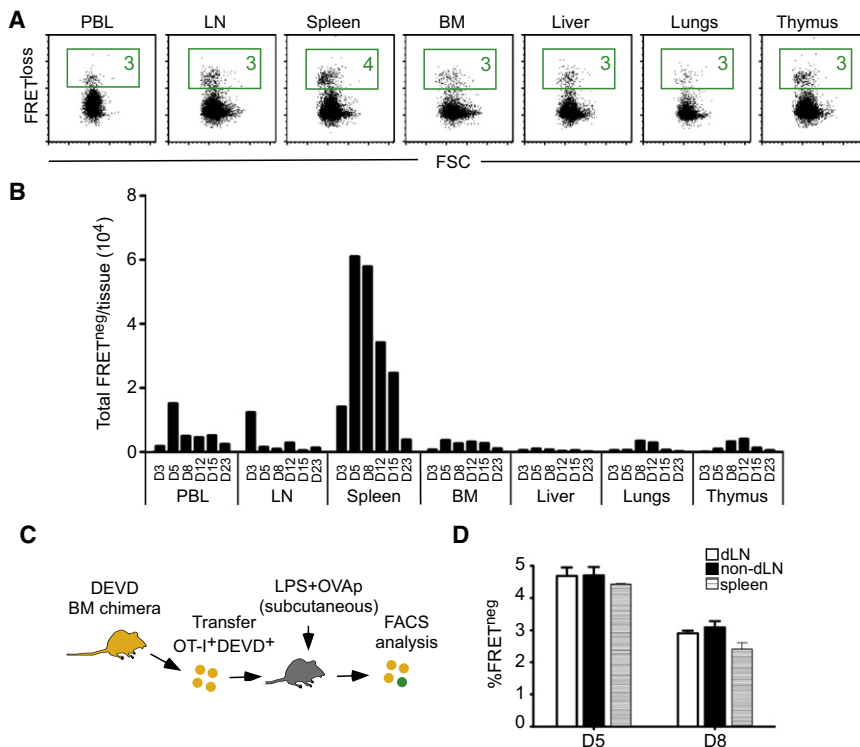
Figure 4. T Cell Contraction Is a Systemic Process
