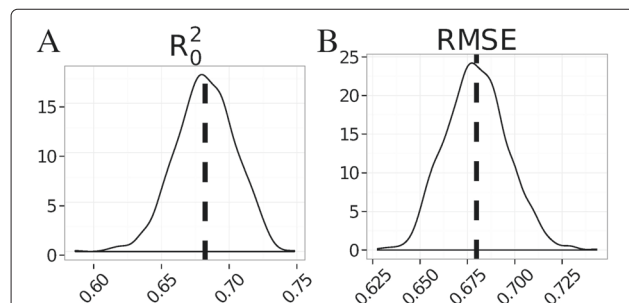
Figure 5 Distribution of theoretical R^2_{0test} (A) and RMSE_{test} (B) values. The mean of the R^2_{0test} distribution, 0.68, highlights that the uncertainty in public bioactivity data does not permit models displaying R^2_{0test} values close to 1. Similar results were obtained for q^2_{test} . From these data we conclude that the minimum RMSE_{test} value that a model can achieve without exhibiting overfitting is close to the experimental uncertainty.
