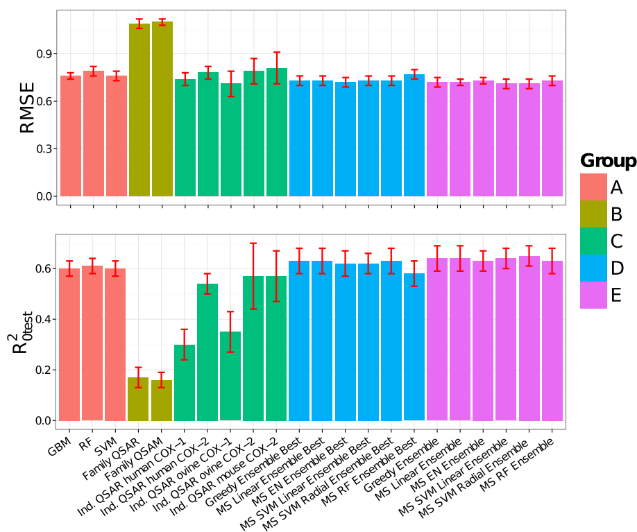
Figure 4 Model performance on the test set. RMSE_{test} (upper panel) and R^2_{0test} (lower panel) values for the following models: (group A) single PCM, (group B) Family QSAR and Family QSAM, (group C) individual QSAR, (group D) model ensembles comprising those single PCM models exhibiting the highest predictive power, and (group E) model ensembles comprising the whole model library. Bars are colored according to the groups defined in Table 2. Confidence intervals correspond to the mean value \pm one standard deviation calculated with bootstrapping [74].
