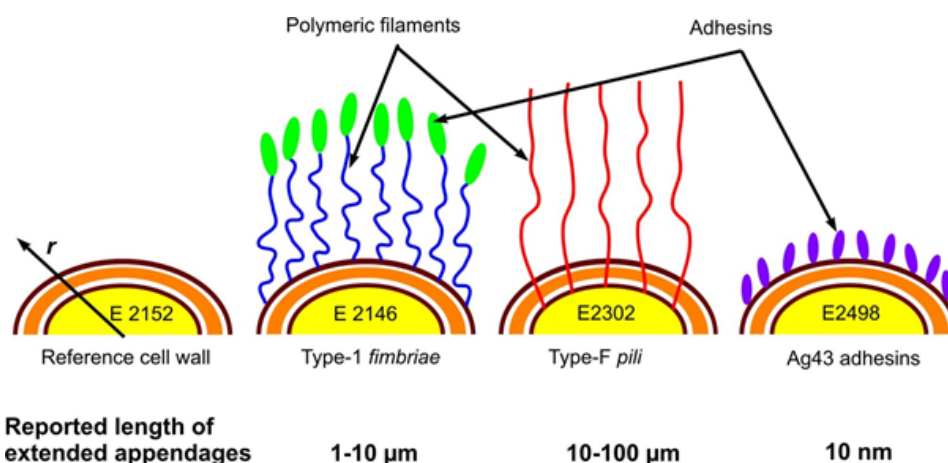
Figure 1. Spatial organization of the external structures for the various E. coli strains investigated. Pili and fimbriae are structures with reported total lengths of about \sim 10\text{--}100\ \mu\text{m} (E2302) and \sim 1\text{--}10\ \mu\text{m} (E2146), respectively, while antigen Ag43 protein layer is a short and rigid structure \sim 10\ \text{nm} thick (E2498).
