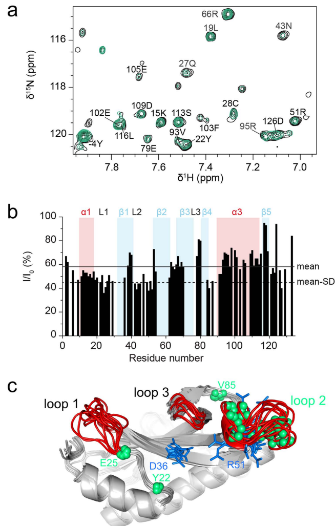
Figure 7. \sigma^S_{STM} -induced perturbations in NMR spectra of CrI_{STM} . (a) Selected region of the ^1H - ^{15}N TROSY spectrum of ^{15}N^2H -labeled CrI_{STM} in the absence (black) and presence of 0.25 equivalents of unlabelled \sigma^S_{STM} (green) showing the intensity decrease of amide signals for some residues like N43. (b) Plot of intensity ratios as a function of residue number. Background colours indicate the boundaries of CrI_{STM} secondary structures (red for \alpha -helices, blue for \beta -strands). The mean value and mean minus one standard deviation (SD) are shown in continuous and dashed lines. (b) The nitrogen atoms of residues with the lowest intensity ratios ( I/I_0 < \text{mean} - \text{SD} ) in the presence of \sigma^S are shown in green spheres on the NMR structure of CrI_{STM} , represented by three conformers to illustrate the structural variability in loop regions (in red). Two critical residues for \sigma^S_{STM} binding, D36 and R51, are represented in blue sticks.
