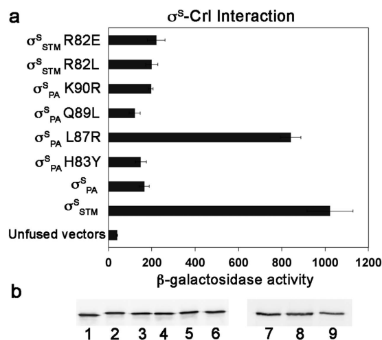
Figure 4. BACTH interaction analyses between CrI from S. Typhimurium and \sigma^S wild-type and variant proteins from S. Typhimurium and P. aeruginosa . (a) Interaction between CrI STM-T18 and the T25- \sigma^S hybrid proteins indicated was quantified by measuring \beta -galactosidase activity in Miller units. Results are the mean of at least three independent experiments and standard deviations are indicated with black bars. (b) Immunodetection of T25- \sigma^S fusion proteins by antibodies directed against the T25 polypeptide. Lane 1, \sigma^S_{STM} ; lane 2, \sigma^S_{PA} ; lane 3, \sigma^S_{PA} H83Y; lane 4, \sigma^S_{PA} L87R; lane 5, \sigma^S_{PA} Q89L; lane 6, \sigma^S_{PA} K90R; lane 7, \sigma^S_{STM} ; lane 8, \sigma^S_{STM} R82L; lane 9, \sigma^S_{STM} R82E.
