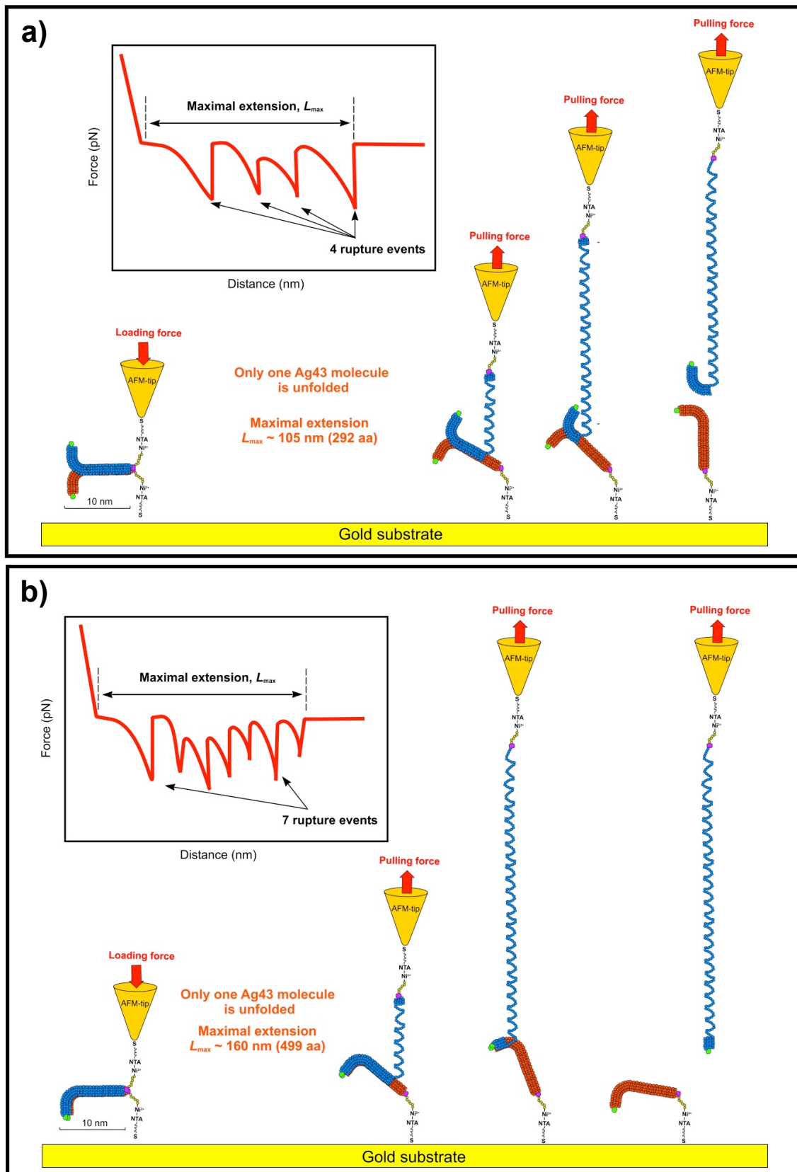
Figure 9. Schematic representation of the unfolding of cis -associated Ag43 \alpha (predominant at sufficiently large values of solution pH and pulling rate).
