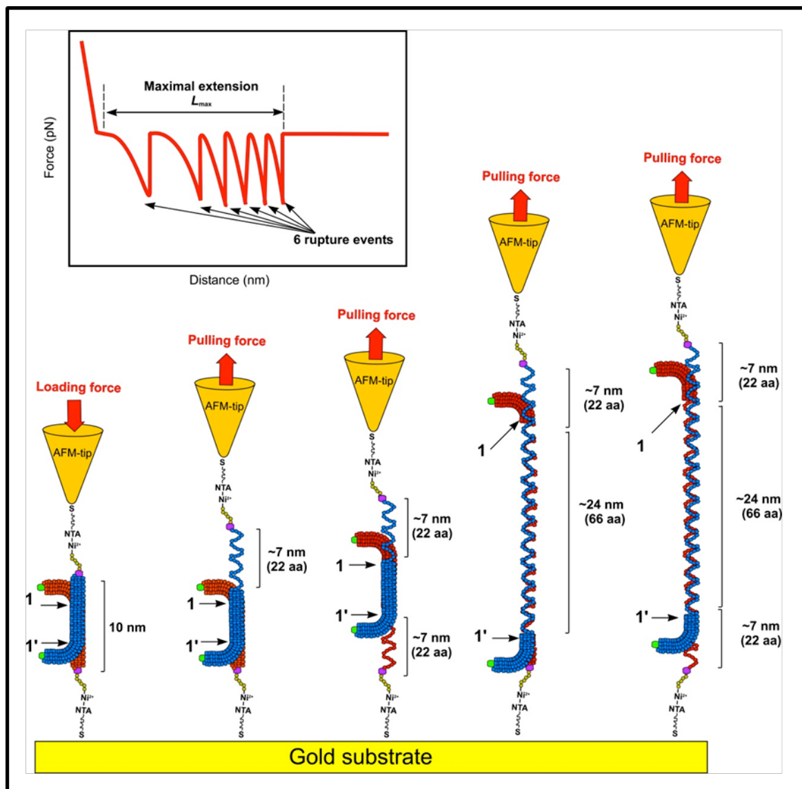
Figure 8. Schematic representation of the unfolding of trans -associated Ag43α (predominant at sufficiently low values of solution pH and pulling rate). Representation of the envisaged unfolding of trans -associated Ag43α dimers formed during force spectroscopy experiments.
