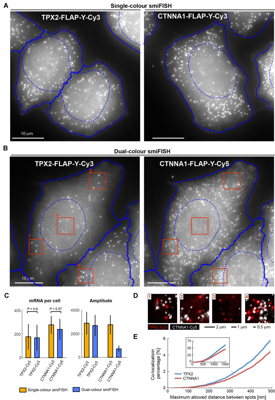
Figure 3. Detection of CTNNA1 and TPX2 mRNA by two-colour smiFISH in HeLa cells. Single-colour smiFISH performed with Cy3 against either gene. Dual-colour smiFISH performed with Cy3 against TPX2, and Cy5 against CTNNA1. Both probe-sets contain FLAP-Y, and were prehybridized separately with the secondary probes before the actual experiment. ( A and B ) Maximum intensity projections of representative smiFISH images for ( A ) single-colour and ( B ) dual-colour experiments. For automated segmentation, nuclei were marked with DAPI, and cells with HCS CellMask TM Green (Molecular Probes). Segmentation was performed on focus-projected images (see last section of results) with CellCognition (10); nuclei shown with dashed blue lines, cells with solid blue lines. ( C ) Left: estimated mRNA number per cell. Reported P -value from Wilcoxon rank sum test for equal medians (Matlab function ranksum ). Right: amplitude of 3D Gaussian fit to each detected mRNA molecule. TPX2 mRNA detection was similar in single-colour and dual-colour experiments with respect to estimated mRNA counts and mRNA spot intensity. Labelling of CTNNA1 mRNA with Cy5 leads to substantially dimmer spots, which makes mRNA detection more challenging and leads to a lower P -value for the comparison of mRNA counts. Number of cells per condition: NCTTNA1 = 143, NTPX2 = 115; NCTTNA1,TPX2 = 150. ( D ) Dual-colour smiFISH (TPX2 in red, and CTNNA1 in white). Images are zoom-ins indicated by red rectangles in ( B ). For better visualization, images were background corrected with the SubtractBackground function in Fiji (Rolling ball radius of 50 pixels). ( E ) Co-localization analysis for dual-colour smiFISH experiment in ( C ). mRNAs were detected in 3D images with FISH-quant (5) and co-localization determined with the Matlab function munkres using the Hungarian Algorithm for linear assignment problems, which is available on Matlab File Exchange. Plots show the co-localization percentage for TPX2 (blue, 27 178 mRNAs) and CTNNA1 (red, 35 623 mRNAs) as a function of the maximum allowed distance between spots to be still considered to be co-localized. For distances smaller than 500 nm, co-localization is smaller than 5%. Larger allowed distances lead to a significant increase of co-localization percentage, since neighbouring spots are erroneously considered to co-localize (especially in denser area such as zoom-in 4).
