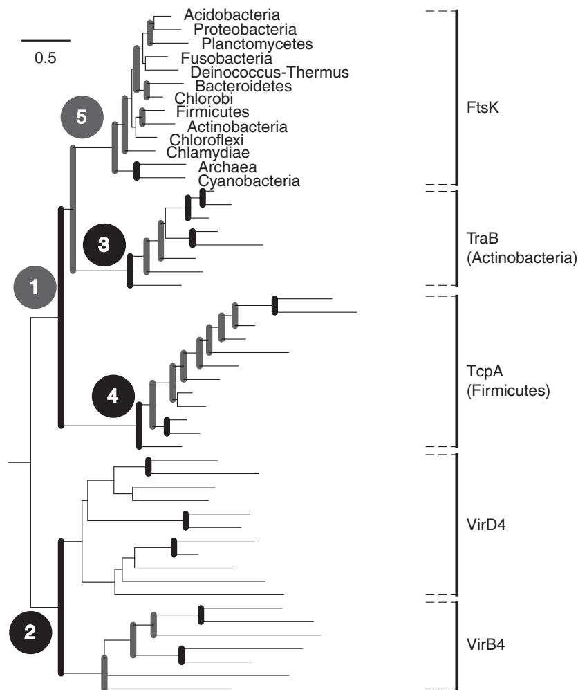
FIG. 2. Phylogenetic analysis of the AAA+ ATPases associated with conjugation. The position of the root was determined using the AAA+ ATPase VirB11 in a separate analysis. Names along the FtsK tips correspond to the taxonomic origins of each protein, reflecting the width of sampling. Bold vertical black lines represent nodes with a high support value (bootstrap >70% and aLRT >0.7). Bold gray lines represent nodes with high aLRT score (>0.7) but a weaker bootstrap (<70%). The homologs of TcpA are found only in Firmicutes. The homologs of TraB are found only in Actinobacteria. Numbers in circles refer to the analysis of robustness in table 1 (identified in the third column of table 1 ); black background stands for a high support ( \geq 70\% bootstrap in the best-scoring alignment) and gray background for a moderate support ( \geq 50\% bootstrap in the best-scoring alignment).
