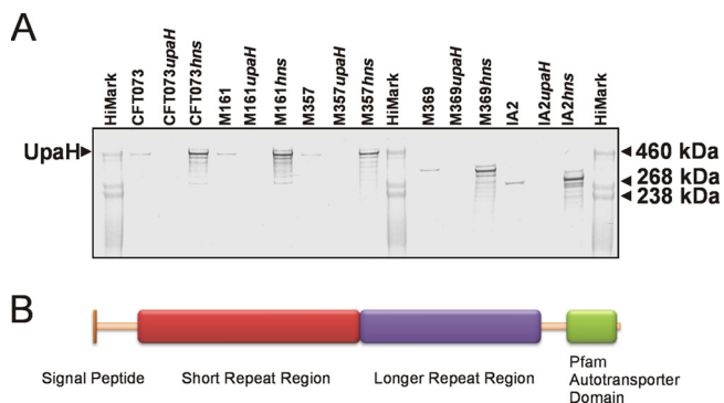
FIG 2 (A) Western blot analysis of UpaH production in whole-cell lysates prepared from E. coli strains CFT073, M161, M357, M369, and IA2 and their respective upaH or hns mutants. (B) Schematic illustration of the domain organization of UpaH from E. coli . Indicated are the signal peptide, the small repeat region, the longer repeat region, and the transmembrane \beta -domain. The repeat regions contain the majority of the sequence differences identified in the UpaH variants.
