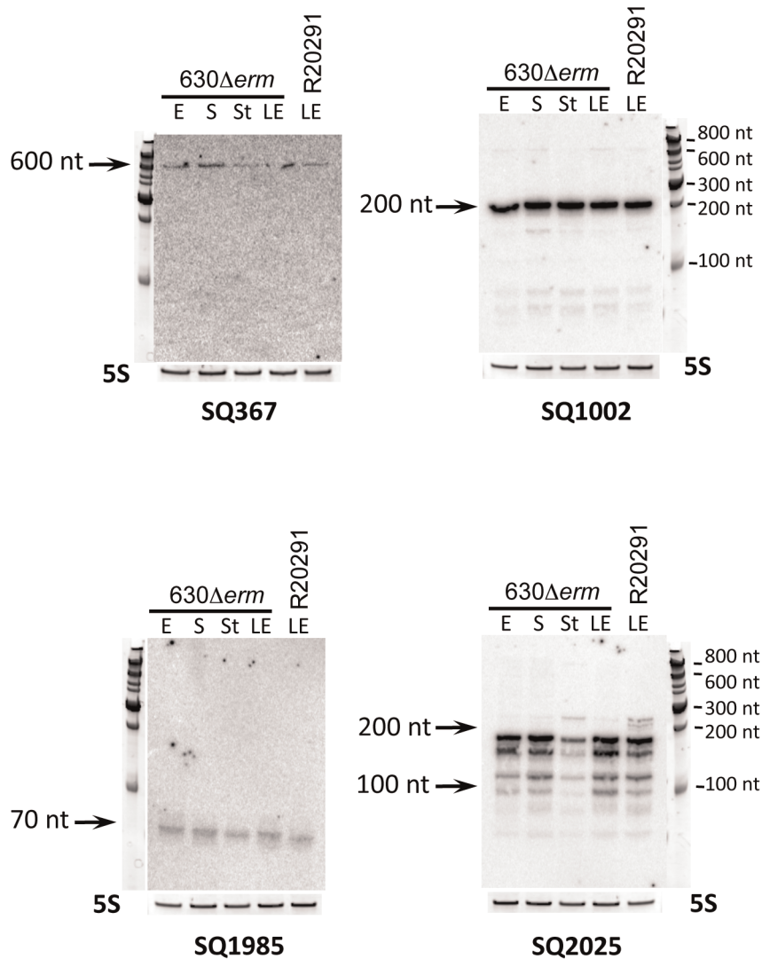
Figure 2. Experimental validation of in silico identified sRNAs. Northern blot was performed for detection of selected sRNAs: SQ367, SQ1002, SQ1985 and SQ2025. RNA samples were extracted from 630Δerm strain grown at exponential phase (E, 4 h of growth), late exponential phase (LE, 6 h of growth), entry to stationary phase (S, 10 h of growth) or under nutrient starvation conditions (St) and from R20291 strain grown at late exponential phase (LE). 5S RNA at the bottom serves as loading control. The arrows show the detected transcripts with their size estimated by comparison with RNA molecular weight standards.
