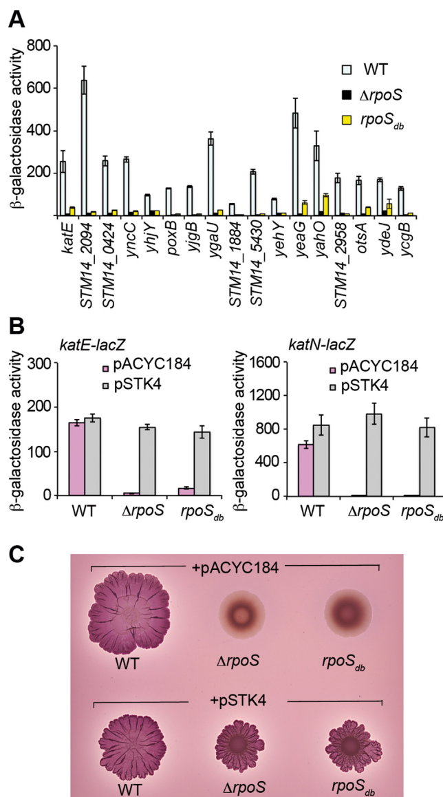
Figure 3. Effects of the \Delta rpoS and rpoS db mutations on \sigma^S -activated genes and the rdar morphotype. (A, B) Expression of transcriptional lacZ fusions in \sigma^S -dependent genes in the wild-type (WT) strain VF7969 and its rpoS derivatives VF9356 and VF9849, grown for 18 h in LB at 37°C. Bar graphs represent the mean \beta -galactosidase activity and error bars represent standard deviation of at least three independent experiments. (C) Development of the red dry and rough ( rdar ) morphotype of the wild-type strain and rpoS mutants carrying the plasmid indicated was visualized on CR plates at 28°C. Empty vector pACYC184 and plasmid pSTK4 carrying the rpoS gene were used in complementation experiments (B, C).
