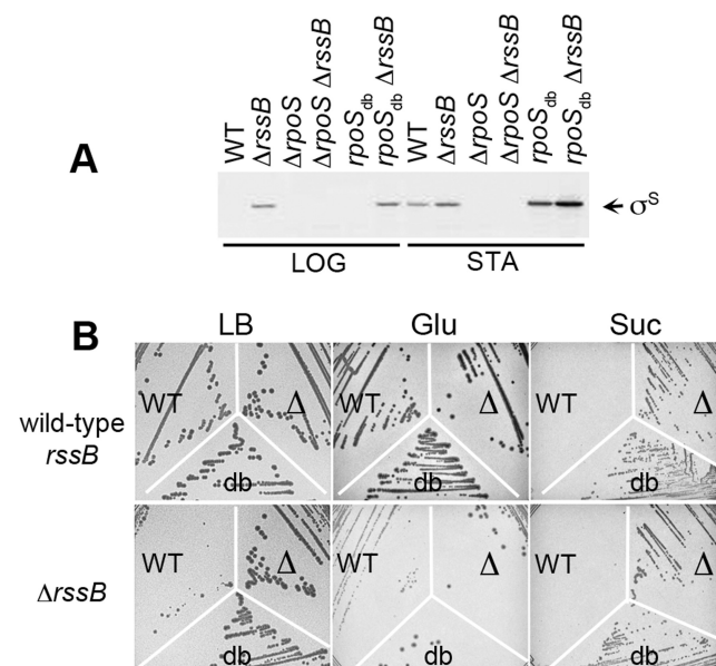
Figure 5. Effect of a \Delta rssB mutation on \sigma^S expression and Salmonella growth. (A) Immunodetection of \sigma^S and \sigma^{S_{db}} in exponential (LOG, OD600 of 0.3) and stationary phase (STA, OD600 of 4.5) LB cultures of the wild-type (WT) strain VF7969 and its rpoS mutants VF9356 and VF9849, carrying wild-type and \Delta rssB alleles. (B) Growth, on LB and minimal medium with succinate (Suc) and glucose (Glu) as a carbon source at 37°C, of the wild-type and \Delta rssB strains carrying a wild-type (WT) or a mutated rpoS allele ( \Delta , deletion of rpoS ; db, rpoS_{db} ).
