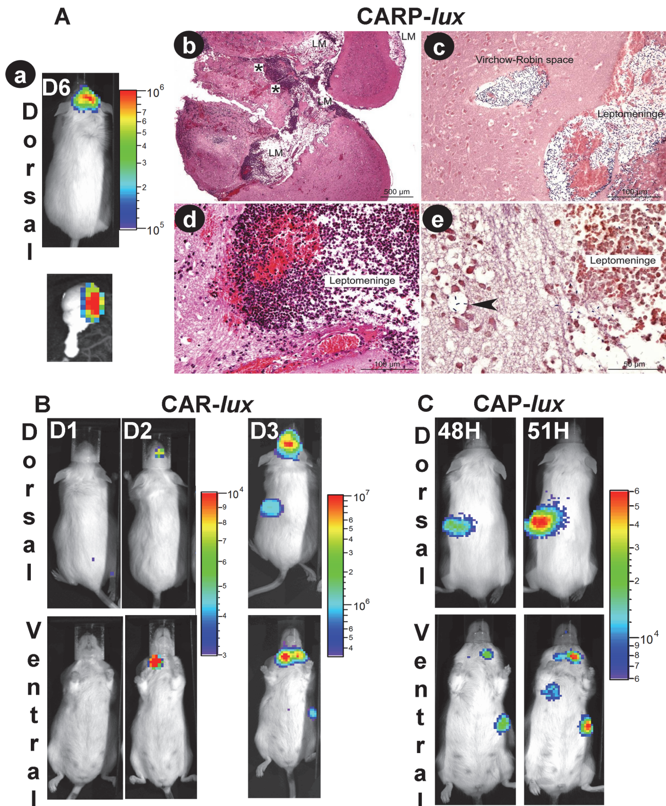
Fig 6. Local role of the HA capsule and in vivo dissemination of the B. cereus bv anthracis CA strain during intranasal infection in mice. Mice were inoculated intranasally with spores of (A) CARP- lux (13 mice, inoculum 1 \times 10^8 ), (B) CAR- lux (16 mice, inoculum 1 \times 10^6 ; all mice died), or (C) CAP- lux (14 mice, inoculum 1 \times 10^6 ; all mice died) strains and bioluminescence was analysed at the indicated times after infection as in Fig 5 (D: days). (Ab-e) Histological characterisation of the infected brain tissue shown in Aa, bottom panel; (Ab) Diffuse inflammatory lesion centred on leptomeninges (LM),
